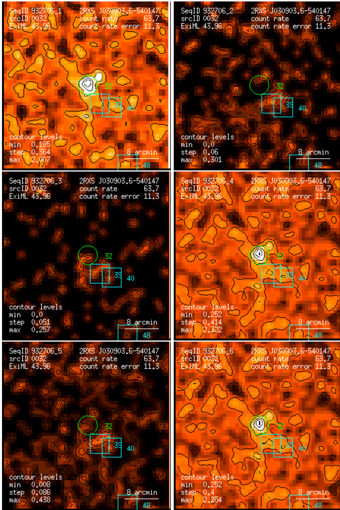
Figure 32: RASS 932706: detection 0032: band rate images, Gaussian filter: (1) PSPC channels 11 – 41, (2) 52 – 90, (3) 91 – 201, (4) 11 – 235, (5) 52 – 201, (6) 11 – 201. Broad band rates in counts/ks. Band rate contour levels in counts/ks/arcmin 2 .
