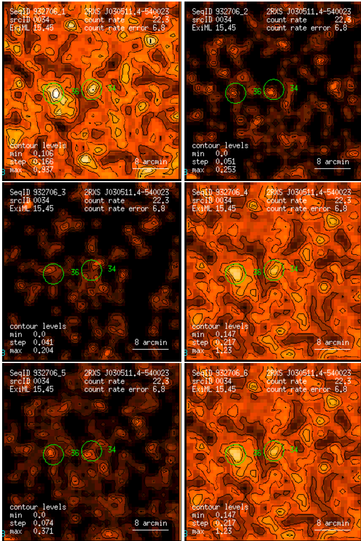
Figure 34: RASS 932706: detection 0034: band rate images, Gaussian filter: (1) PSPC channels 11 – 41, (2) 52 – 90, (3) 91 – 201, (4) 11 – 235, (5) 52 – 201, (6) 11 – 201. Broad band rates in counts/ks. Band rate contour levels in counts/ks/arcmin 2 .
