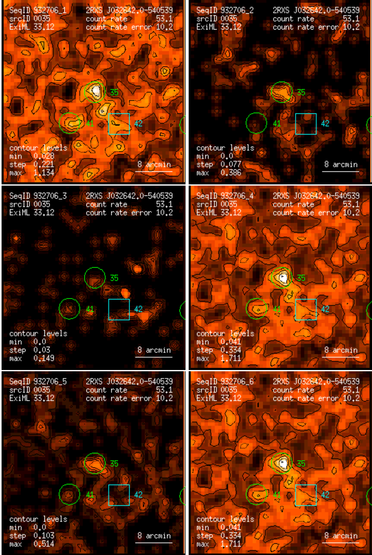
Figure 35: RASS 932706: detection 0035: band rate images, Gaussian filter: (1) PSPC channels 11 – 41, (2) 52 – 90, (3) 91 – 201, (4) 11 – 235, (5) 52 – 201, (6) 11 – 201. Broad band rates in counts/ks. Band rate contour levels in counts/ks/arcmin 2 .
