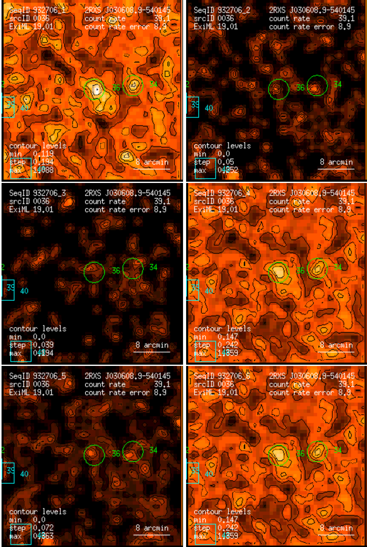
Figure 36: RASS 932706: detection 0036: band rate images, Gaussian filter: (1) PSPC channels 11 – 41, (2) 52 – 90, (3) 91 – 201, (4) 11 – 235, (5) 52 – 201, (6) 11 – 201. Broad band rates in counts/ks. Band rate contour levels in counts/ks/arcmin 2 .
