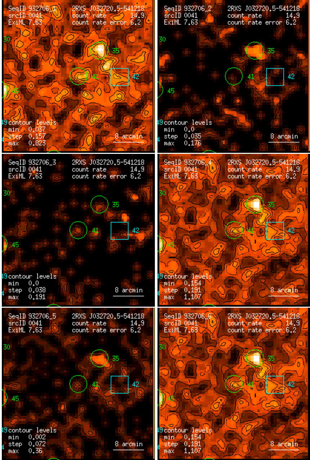
Figure 41: RASS 932706: detection 0041: band rate images, Gaussian filter: (1) PSPC channels 11 – 41, (2) 52 – 90, (3) 91 – 201, (4) 11 – 235, (5) 52 – 201, (6) 11 – 201. Broad band rates in counts/ks. Band rate contour levels in counts/ks/arcmin 2 .
