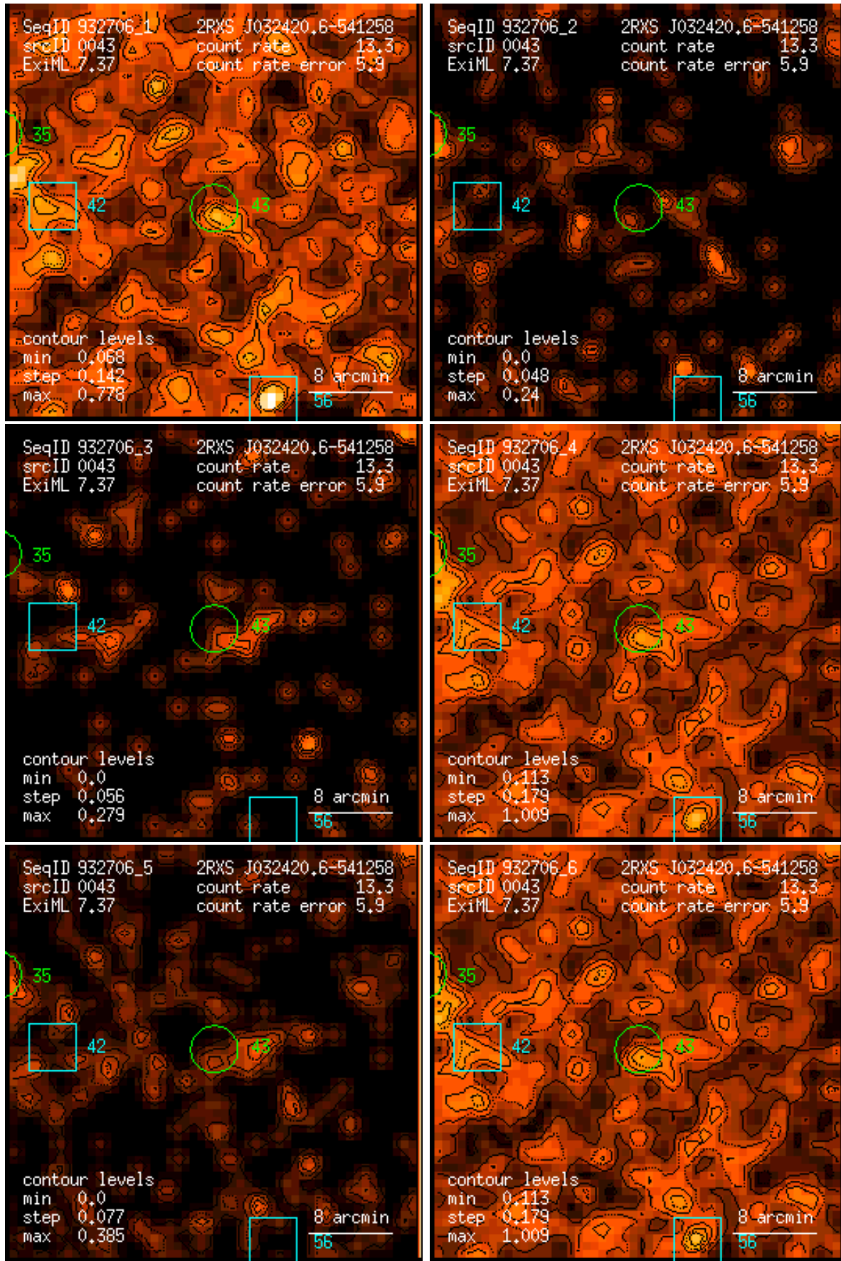
Figure 43: RASS 932706: detection 0043: band rate images, Gaussian filter: (1) PSPC channels 11 – 41, (2) 52 – 90, (3) 91 – 201, (4) 11 – 235, (5) 52 – 201, (6) 11 – 201. Broad band rates in counts/ks. Band rate contour levels in counts/ks/arcmin 2 .
