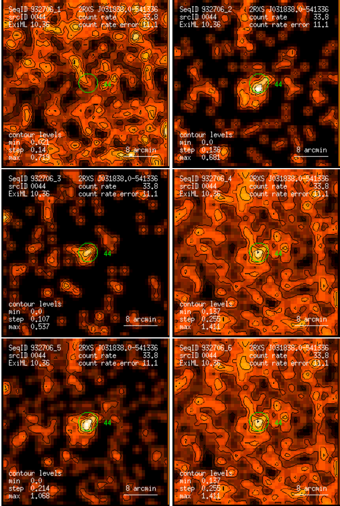
Figure 44: RASS 932706: detection 0044: band rate images, Gaussian filter: (1) PSPC channels 11 – 41, (2) 52 – 90, (3) 91 – 201, (4) 11 – 235, (5) 52 – 201, (6) 11 – 201. Broad band rates in counts/ks. Band rate contour levels in counts/ks/arcmin 2 .
