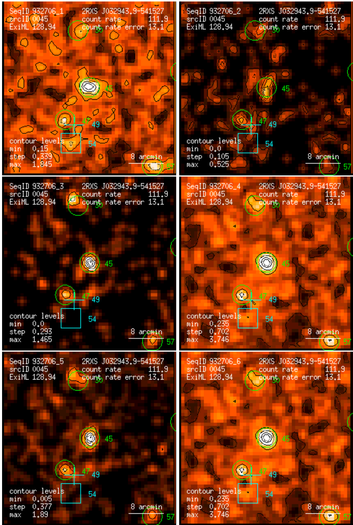
Figure 45: RASS 932706: detection 0045: band rate images, Gaussian filter: (1) PSPC channels 11 – 41, (2) 52 – 90, (3) 91 – 201, (4) 11 – 235, (5) 52 – 201, (6) 11 – 201. Broad band rates in counts/ks. Band rate contour levels in counts/ks/arcmin 2 .
