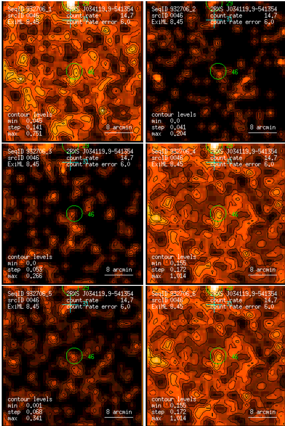
Figure 46: RASS 932706: detection 0046: band rate images, Gaussian filter: (1) PSPC channels 11 – 41, (2) 52 – 90, (3) 91 – 201, (4) 11 – 235, (5) 52 – 201, (6) 11 – 201. Broad band rates in counts/ks. Band rate contour levels in counts/ks/arcmin 2 .
