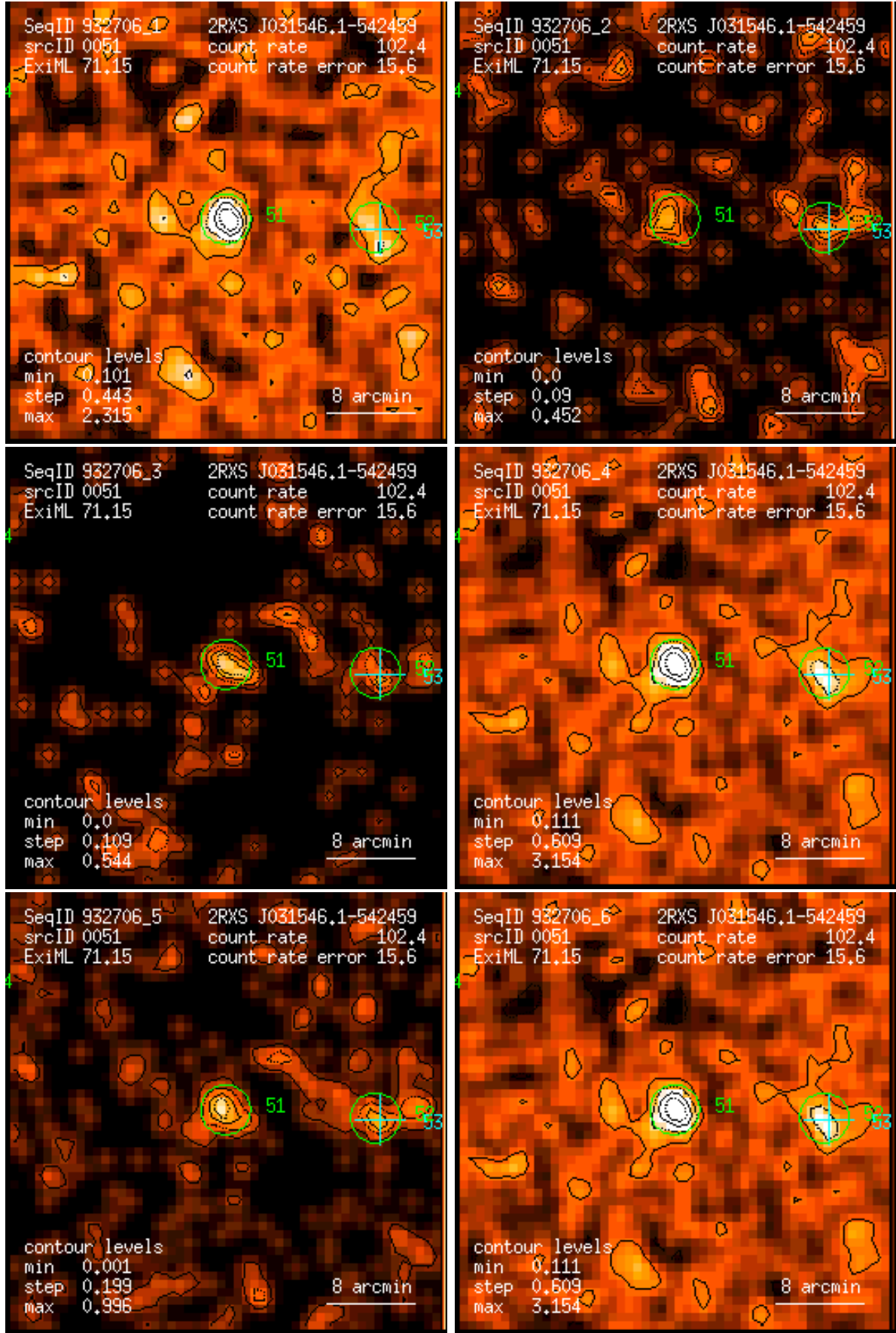
Figure 51: RASS 932706: detection 0051: band rate images, Gaussian filter: (1) PSPC channels 11 – 41, (2) 52 – 90, (3) 91 – 201, (4) 11 – 235, (5) 52 – 201, (6) 11 – 201. Broad band rates in counts/ks. Band rate contour levels in counts/ks/arcmin 2 .
