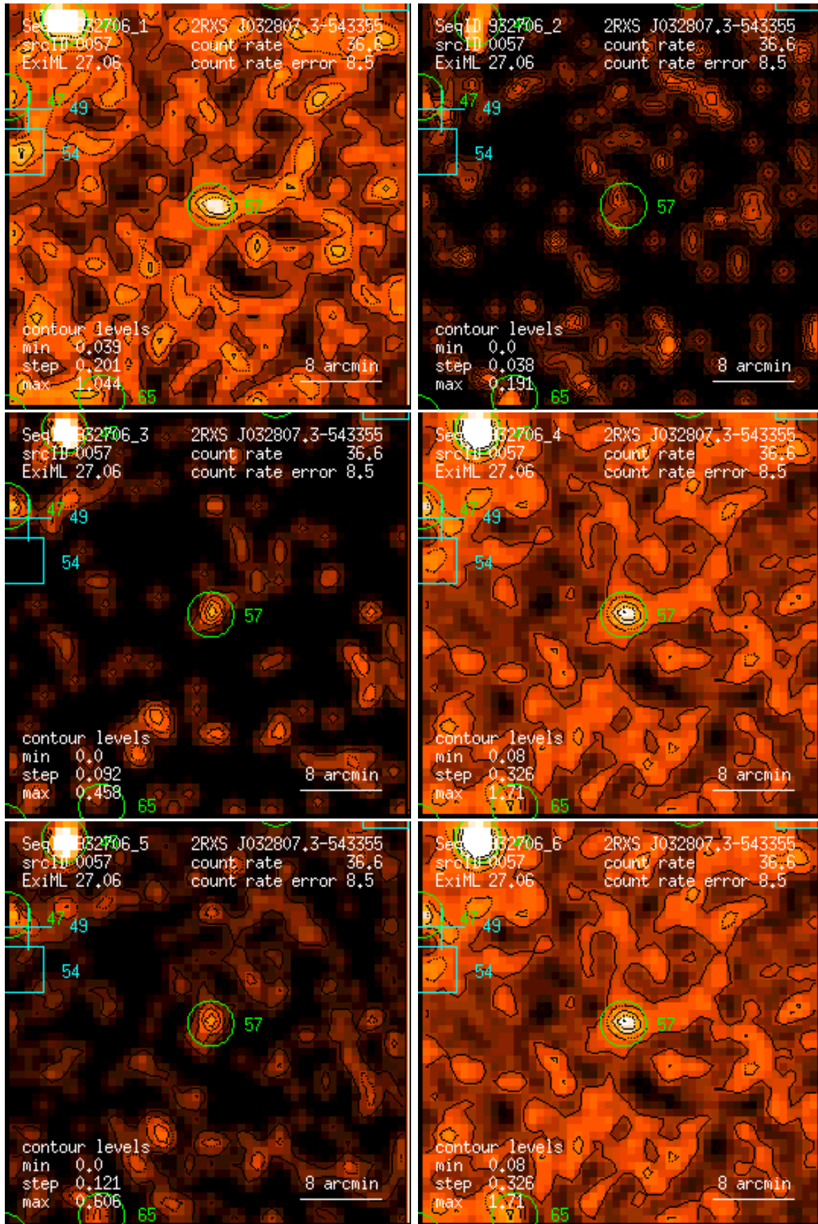
Figure 57: RASS 932706: detection 0057: band rate images, Gaussian filter: (1) PSPC channels 11 – 41, (2) 52 – 90, (3) 91 – 201, (4) 11 – 235, (5) 52 – 201, (6) 11 – 201. Broad band rates in counts/ks. Band rate contour levels in counts/ks/arcmin 2 .
