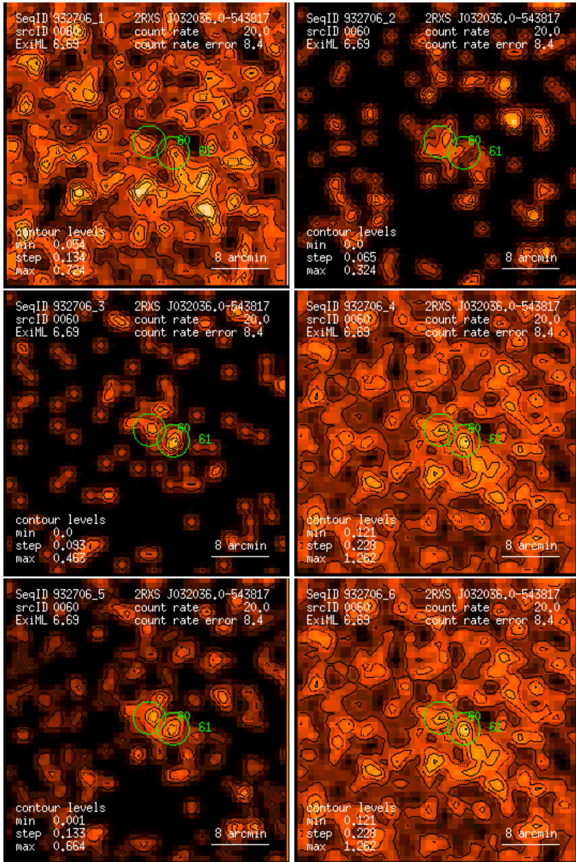
Figure 60: RASS 932706: detection 0060: band rate images, Gaussian filter: (1) PSPC channels 11 – 41, (2) 52 – 90, (3) 91 – 201, (4) 11 – 235, (5) 52 – 201, (6) 11 – 201. Broad band rates in counts/ks. Band rate contour levels in counts/ks/arcmin 2 .
