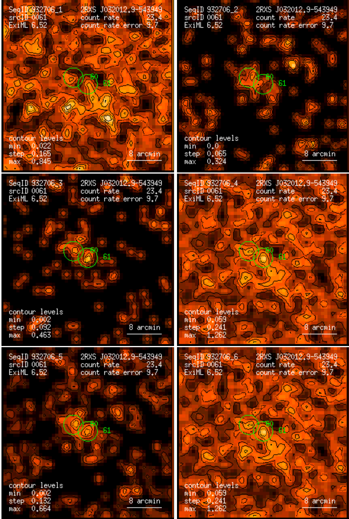
Figure 61: RASS 932706: detection 0061: band rate images, Gaussian filter: (1) PSPC channels 11 – 41, (2) 52 – 90, (3) 91 – 201, (4) 11 – 235, (5) 52 – 201, (6) 11 – 201. Broad band rates in counts/ks. Band rate contour levels in counts/ks/arcmin 2 .
