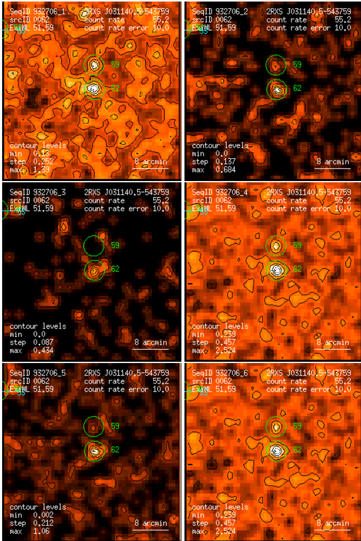
Figure 62: RASS 932706: detection 0062: band rate images, Gaussian filter: (1) PSPC channels 11 – 41, (2) 52 – 90, (3) 91 – 201, (4) 11 – 235, (5) 52 – 201, (6) 11 – 201. Broad band rates in counts/ks. Band rate contour levels in counts/ks/arcmin 2 .
