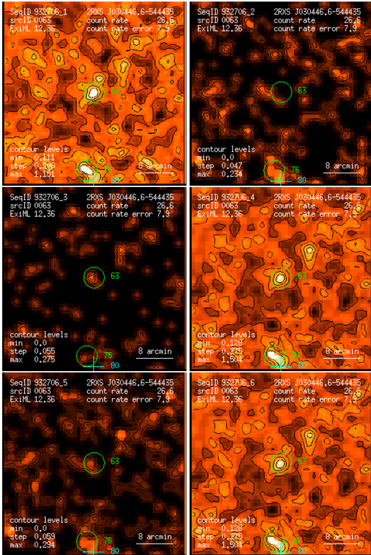
Figure 63: RASS 932706: detection 0063: band rate images, Gaussian filter: (1) PSPC channels 11 – 41, (2) 52 – 90, (3) 91 – 201, (4) 11 – 235, (5) 52 – 201, (6) 11 – 201. Broad band rates in counts/ks. Band rate contour levels in counts/ks/arcmin 2 .
