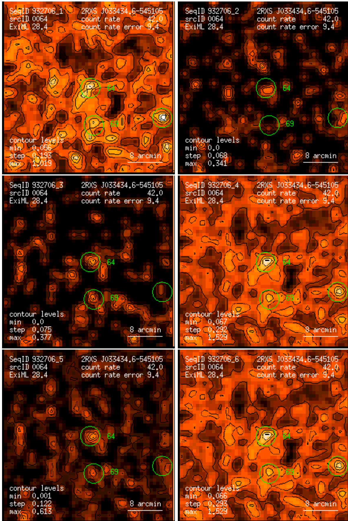
Figure 64: RASS 932706: detection 0064: band rate images, Gaussian filter: (1) PSPC channels 11 – 41, (2) 52 – 90, (3) 91 – 201, (4) 11 – 235, (5) 52 – 201, (6) 11 – 201. Broad band rates in counts/ks. Band rate contour levels in counts/ks/arcmin 2 .
