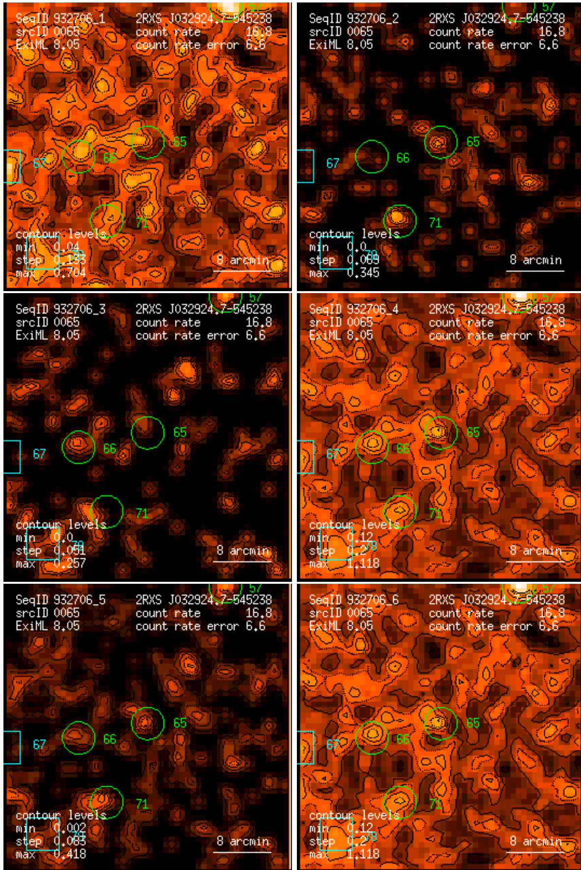
Figure 65: RASS 932706: detection 0065: band rate images, Gaussian filter: (1) PSPC channels 11 – 41, (2) 52 – 90, (3) 91 – 201, (4) 11 – 235, (5) 52 – 201, (6) 11 – 201. Broad band rates in counts/ks. Band rate contour levels in counts/ks/arcmin 2 .
