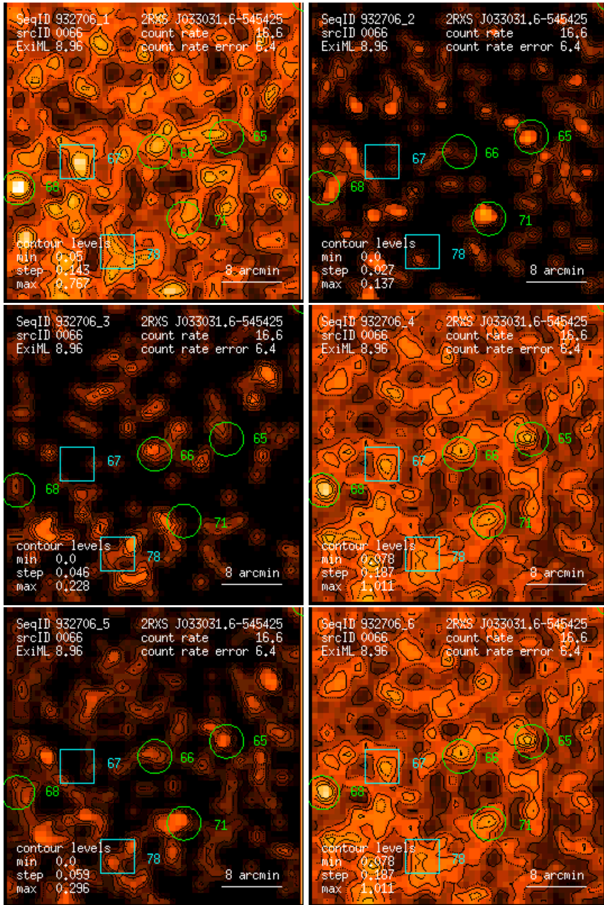
Figure 66: RASS 932706: detection 0066: band rate images, Gaussian filter: (1) PSPC channels 11 – 41, (2) 52 – 90, (3) 91 – 201, (4) 11 – 235, (5) 52 – 201, (6) 11 – 201. Broad band rates in counts/ks. Band rate contour levels in counts/ks/arcmin 2 .
