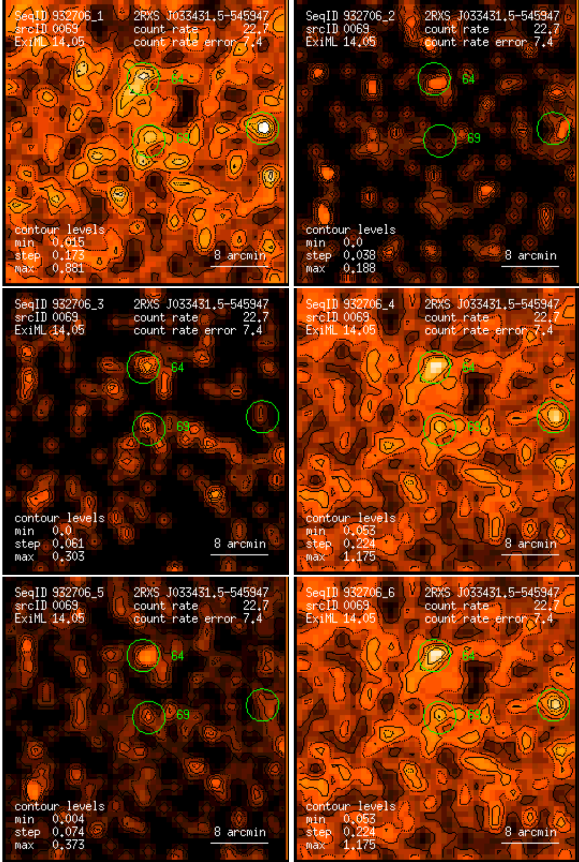
Figure 69: RASS 932706: detection 0069: band rate images, Gaussian filter: (1) PSPC channels 11 – 41, (2) 52 – 90, (3) 91 – 201, (4) 11 – 235, (5) 52 – 201, (6) 11 – 201. Broad band rates in counts/ks. Band rate contour levels in counts/ks/arcmin 2 .
