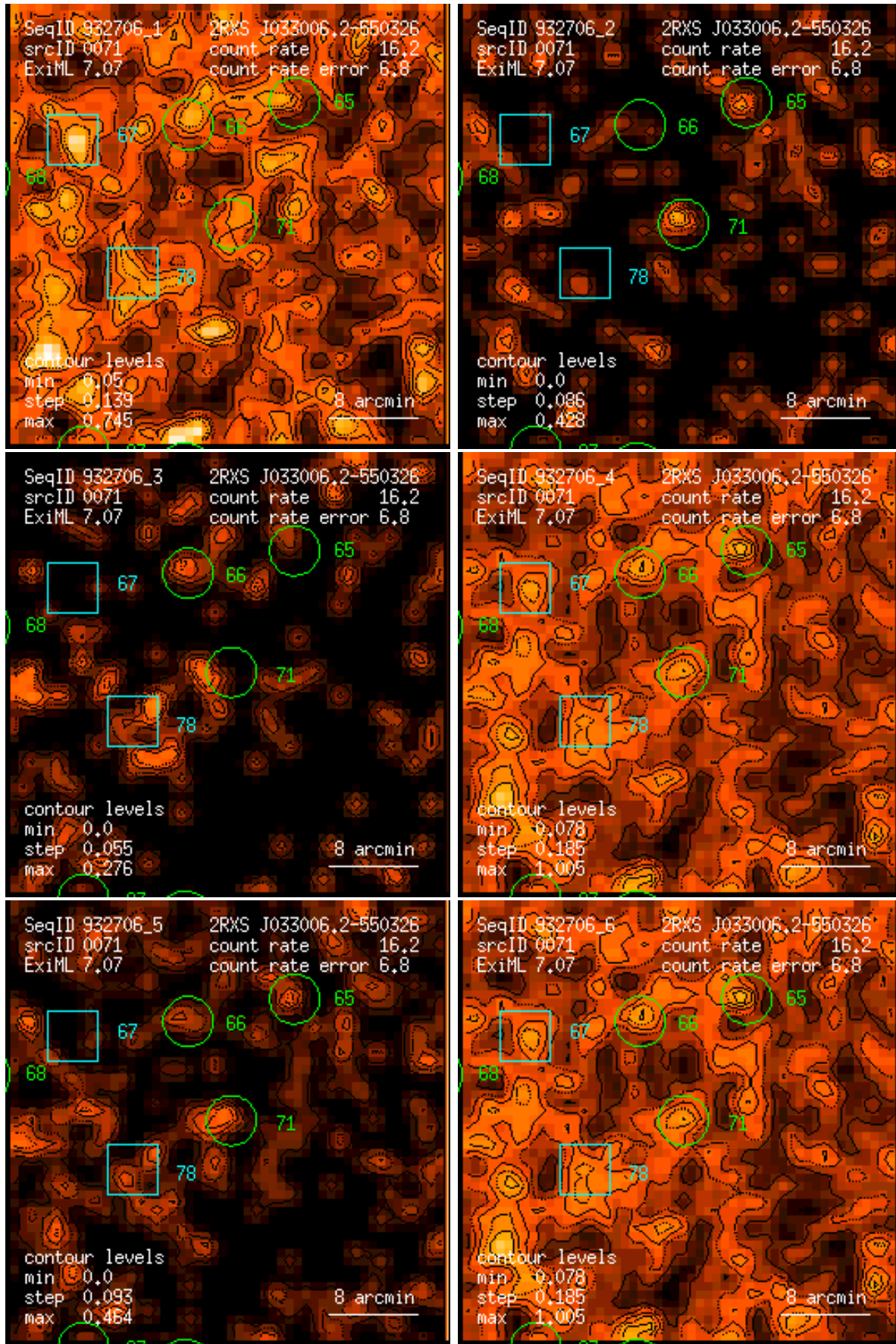
Figure 71: RASS 932706: detection 0071: band rate images, Gaussian filter: (1) PSPC channels 11 – 41, (2) 52 – 90, (3) 91 – 201, (4) 11 – 235, (5) 52 – 201, (6) 11 – 201. Broad band rates in counts/ks. Band rate contour levels in counts/ks/arcmin 2 .
