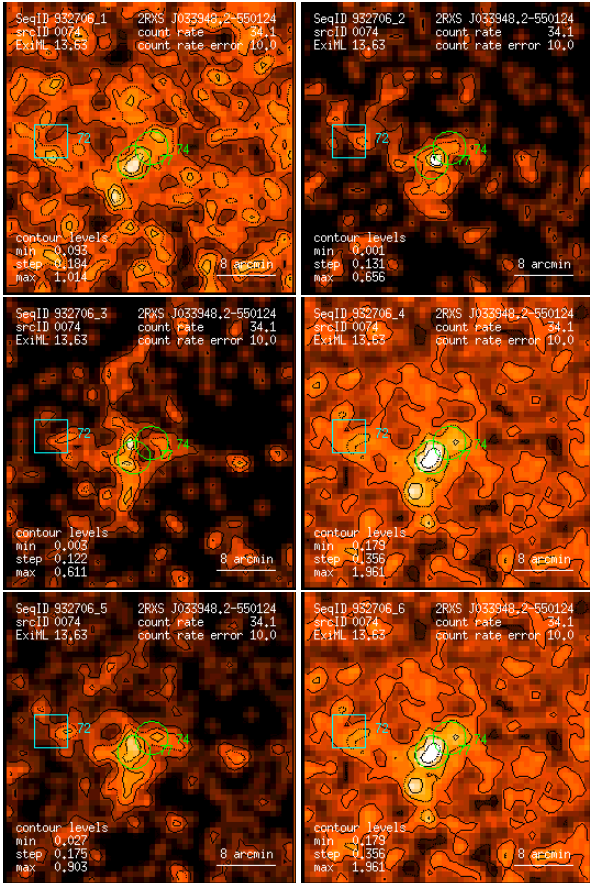
Figure 74: RASS 932706: detection 0074: band rate images, Gaussian filter: (1) PSPC channels 11 – 41, (2) 52 – 90, (3) 91 – 201, (4) 11 – 235, (5) 52 – 201, (6) 11 – 201. Broad band rates in counts/ks. Band rate contour levels in counts/ks/arcmin 2 .
