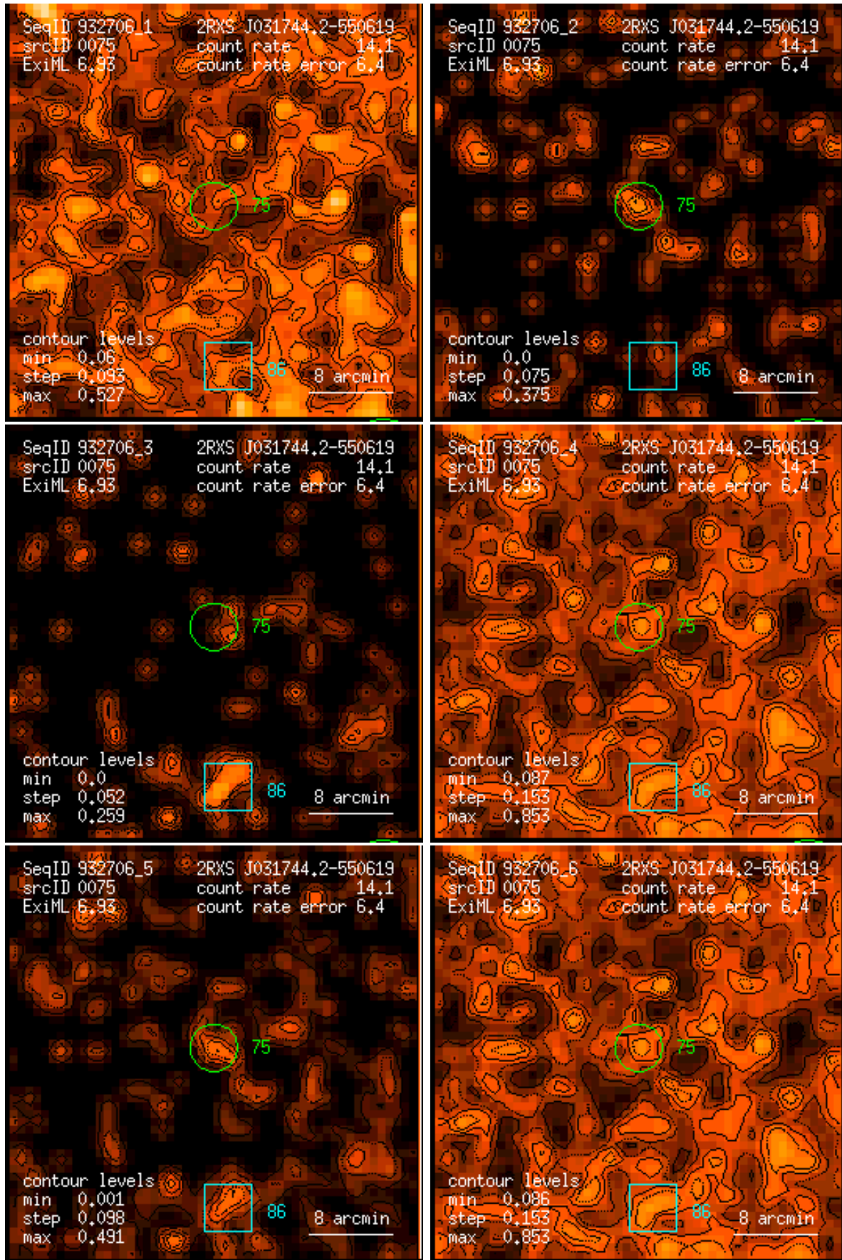
Figure 75: RASS 932706: detection 0075: band rate images, Gaussian filter: (1) PSPC channels 11 – 41, (2) 52 – 90, (3) 91 – 201, (4) 11 – 235, (5) 52 – 201, (6) 11 – 201. Broad band rates in counts/ks. Band rate contour levels in counts/ks/arcmin 2 .
