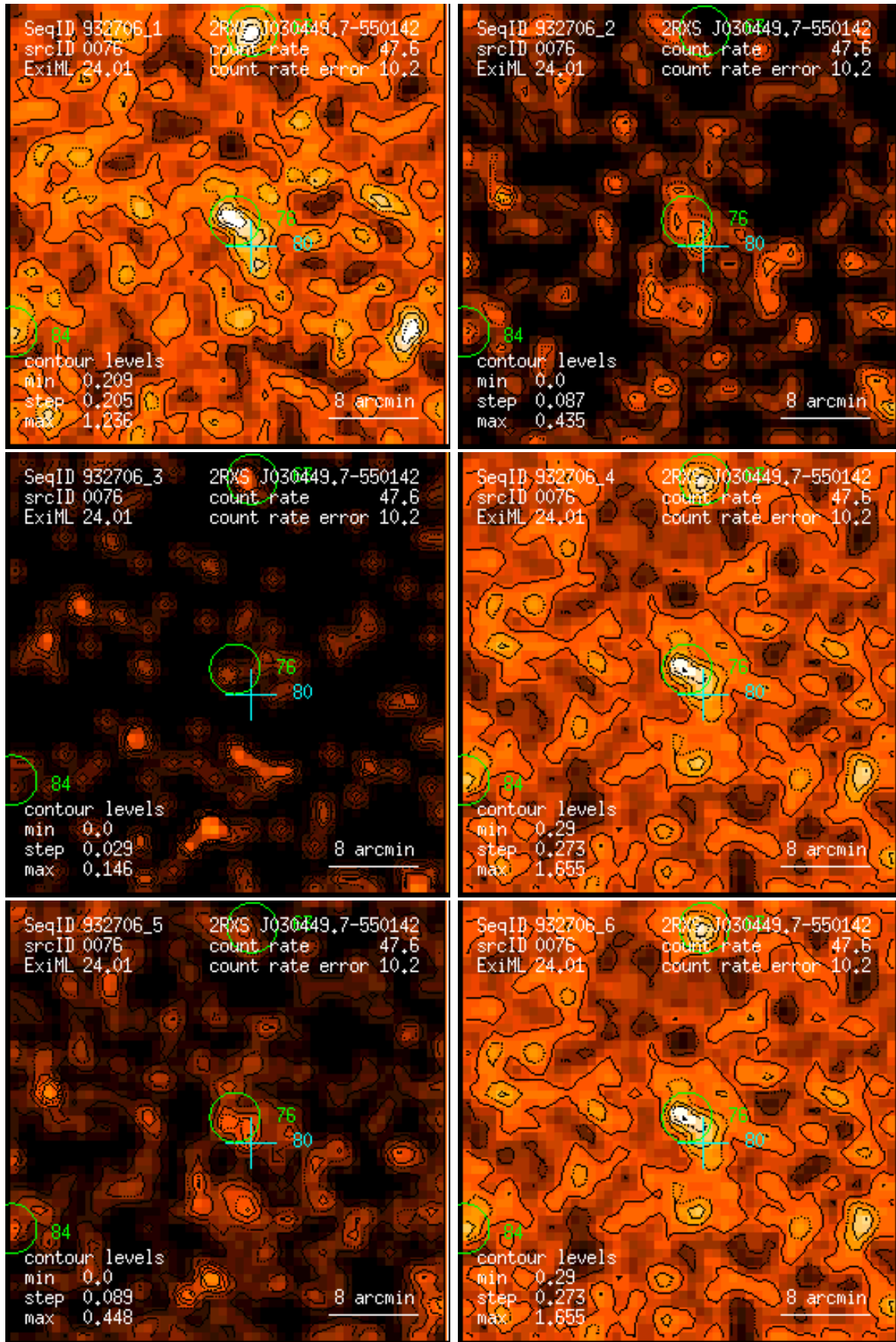
Figure 76: RASS 932706: detection 0076: band rate images, Gaussian filter: (1) PSPC channels 11 – 41, (2) 52 – 90, (3) 91 – 201, (4) 11 – 235, (5) 52 – 201, (6) 11 – 201. Broad band rates in counts/ks. Band rate contour levels in counts/ks/arcmin 2 .
