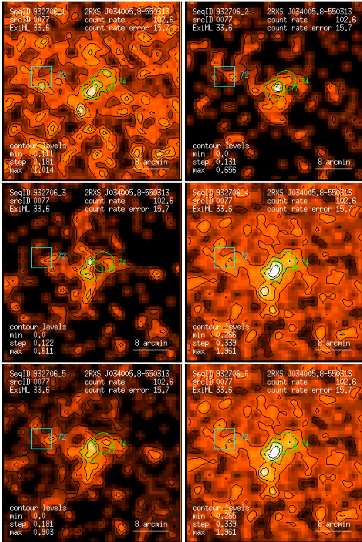
Figure 77: RASS 932706: detection 0077: band rate images, Gaussian filter: (1) PSPC channels 11 – 41, (2) 52 – 90, (3) 91 – 201, (4) 11 – 235, (5) 52 – 201, (6) 11 – 201. Broad band rates in counts/ks. Band rate contour levels in counts/ks/arcmin 2 .
