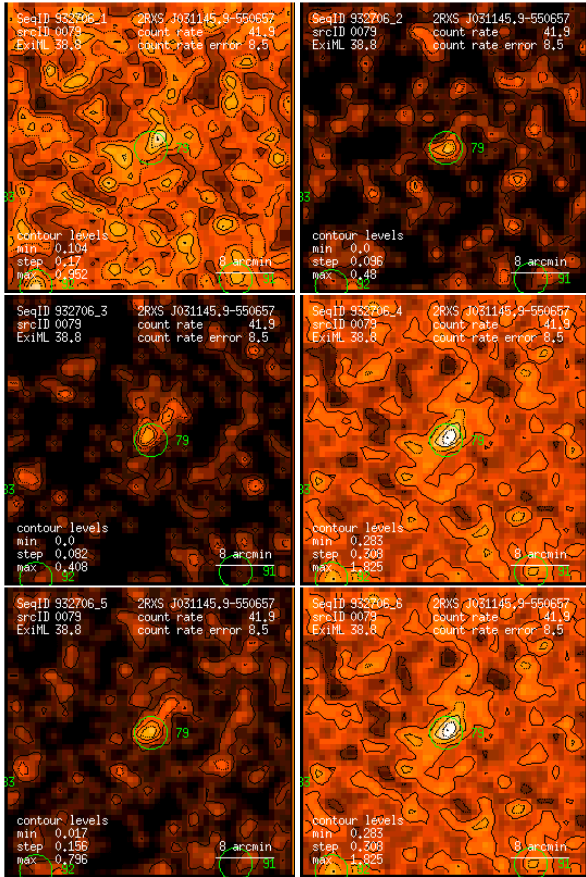
Figure 79: RASS 932706: detection 0079: band rate images, Gaussian filter: (1) PSPC channels 11 – 41, (2) 52 – 90, (3) 91 – 201, (4) 11 – 235, (5) 52 – 201, (6) 11 – 201. Broad band rates in counts/ks. Band rate contour levels in counts/ks/arcmin 2 .
