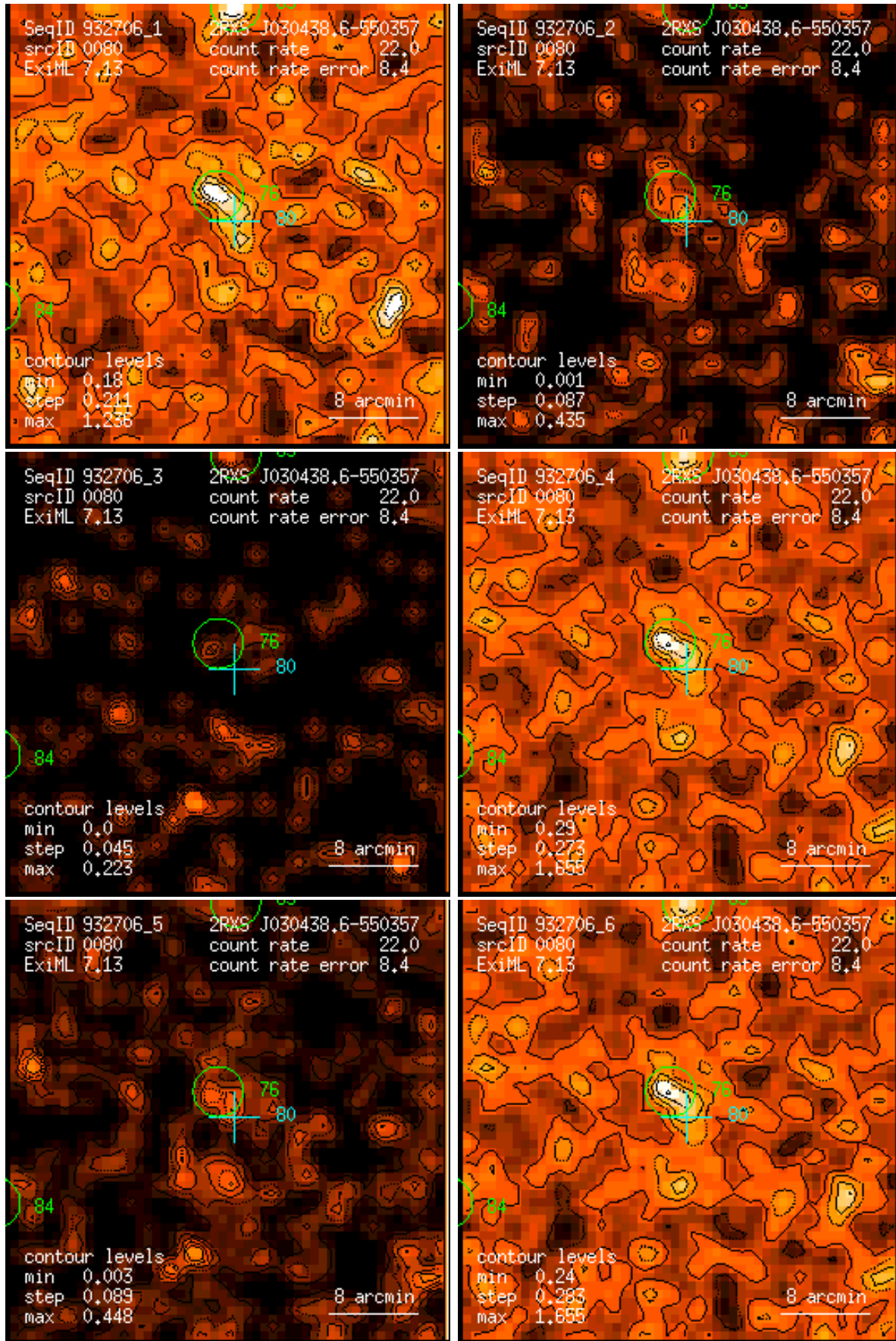
Figure 80: RASS 932706: detection 0080: band rate images, Gaussian filter: (1) PSPC channels 11 – 41, (2) 52 – 90, (3) 91 – 201, (4) 11 – 235, (5) 52 – 201, (6) 11 – 201. Broad band rates in counts/ks. Band rate contour levels in counts/ks/arcmin 2 .
