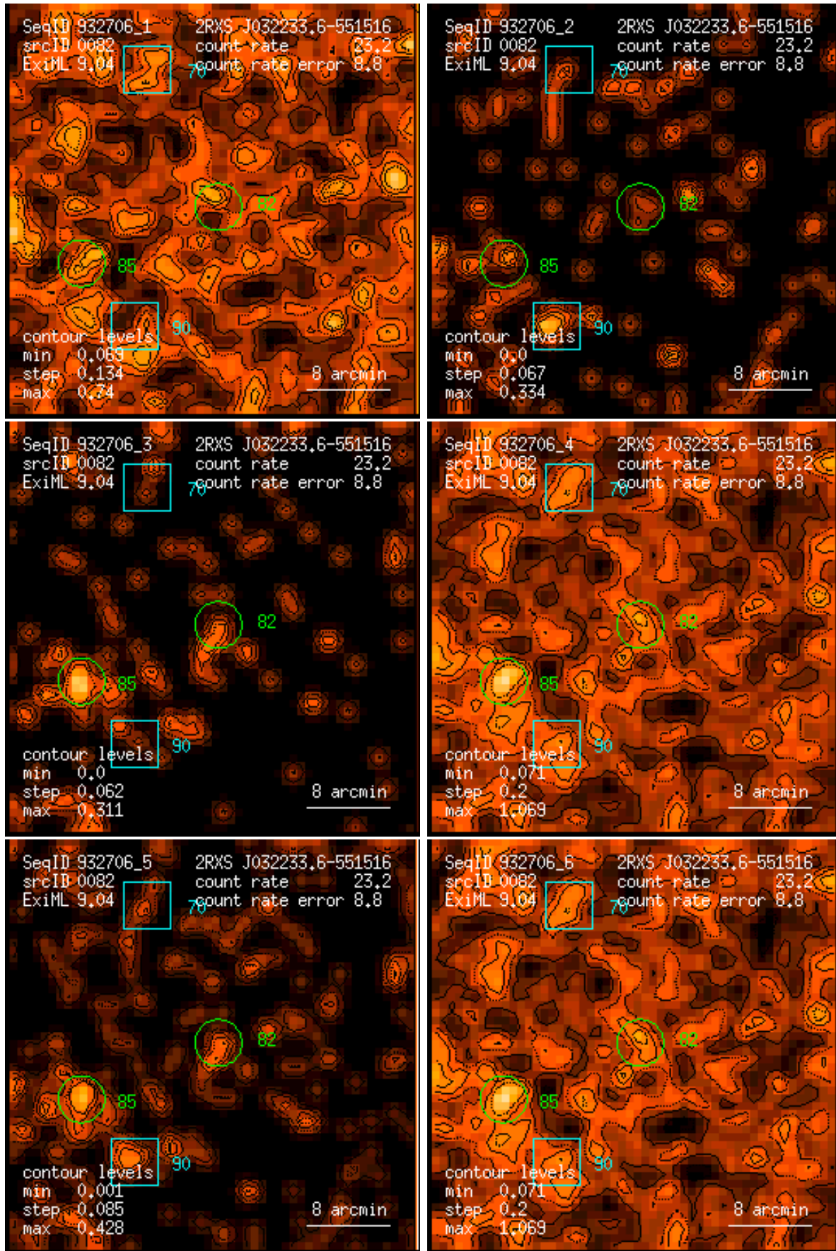
Figure 82: RASS 932706: detection 0082: band rate images, Gaussian filter: (1) PSPC channels 11 – 41, (2) 52 – 90, (3) 91 – 201, (4) 11 – 235, (5) 52 – 201, (6) 11 – 201. Broad band rates in counts/ks. Band rate contour levels in counts/ks/arcmin 2 .
