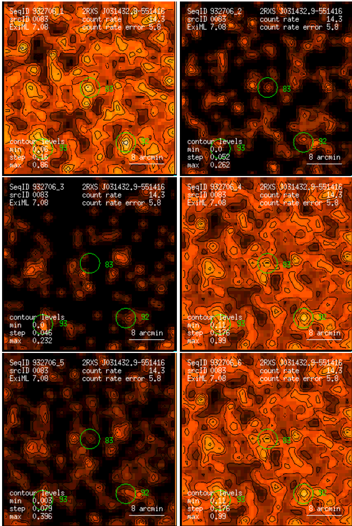
Figure 83: RASS 932706: detection 0083: band rate images, Gaussian filter: (1) PSPC channels 11 – 41, (2) 52 – 90, (3) 91 – 201, (4) 11 – 235, (5) 52 – 201, (6) 11 – 201. Broad band rates in counts/ks. Band rate contour levels in counts/ks/arcmin 2 .
