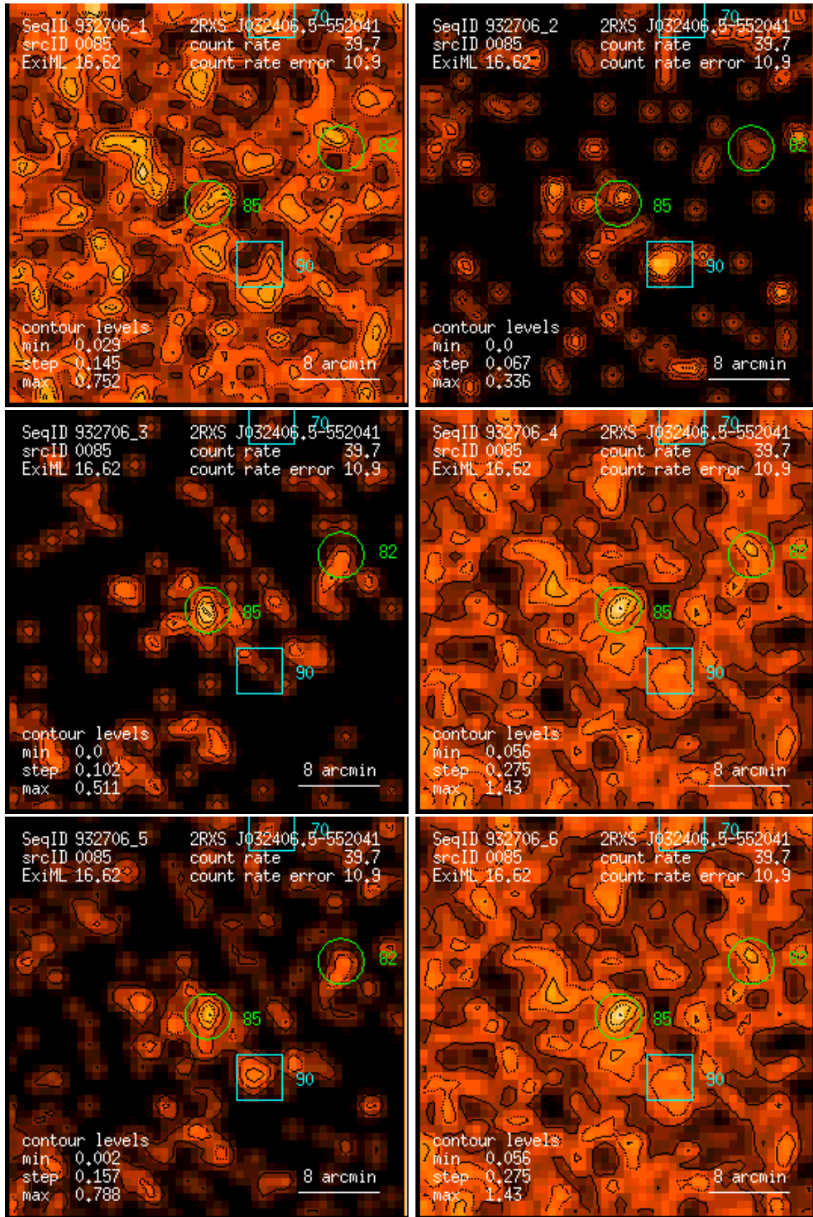
Figure 85: RASS 932706: detection 0085: band rate images, Gaussian filter: (1) PSPC channels 11 – 41, (2) 52 – 90, (3) 91 – 201, (4) 11 – 235, (5) 52 – 201, (6) 11 – 201. Broad band rates in counts/ks. Band rate contour levels in counts/ks/arcmin 2 .
