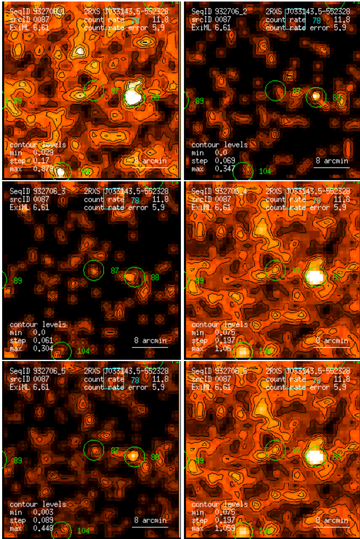
Figure 87: RASS 932706: detection 0087: band rate images, Gaussian filter: (1) PSPC channels 11 – 41, (2) 52 – 90, (3) 91 – 201, (4) 11 – 235, (5) 52 – 201, (6) 11 – 201. Broad band rates in counts/ks. Band rate contour levels in counts/ks/arcmin 2 .
