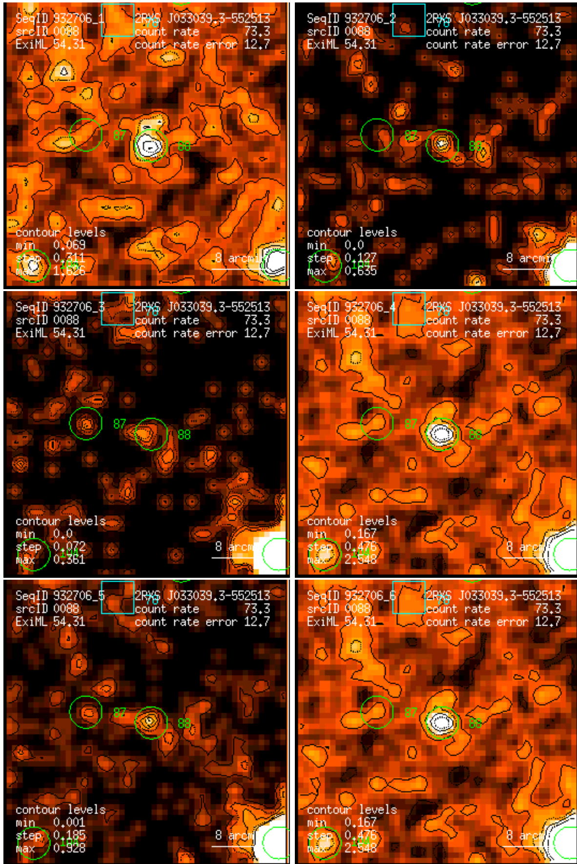
Figure 88: RASS 932706: detection 0088: band rate images, Gaussian filter: (1) PSPC channels 11 – 41, (2) 52 – 90, (3) 91 – 201, (4) 11 – 235, (5) 52 – 201, (6) 11 – 201. Broad band rates in counts/ks. Band rate contour levels in counts/ks/arcmin 2 .
