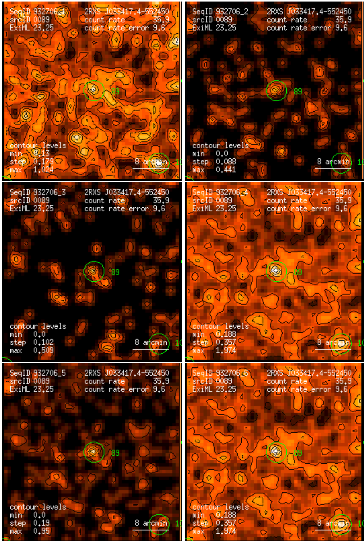
Figure 89: RASS 932706: detection 0089: band rate images, Gaussian filter: (1) PSPC channels 11 – 41, (2) 52 – 90, (3) 91 – 201, (4) 11 – 235, (5) 52 – 201, (6) 11 – 201. Broad band rates in counts/ks. Band rate contour levels in counts/ks/arcmin 2 .
