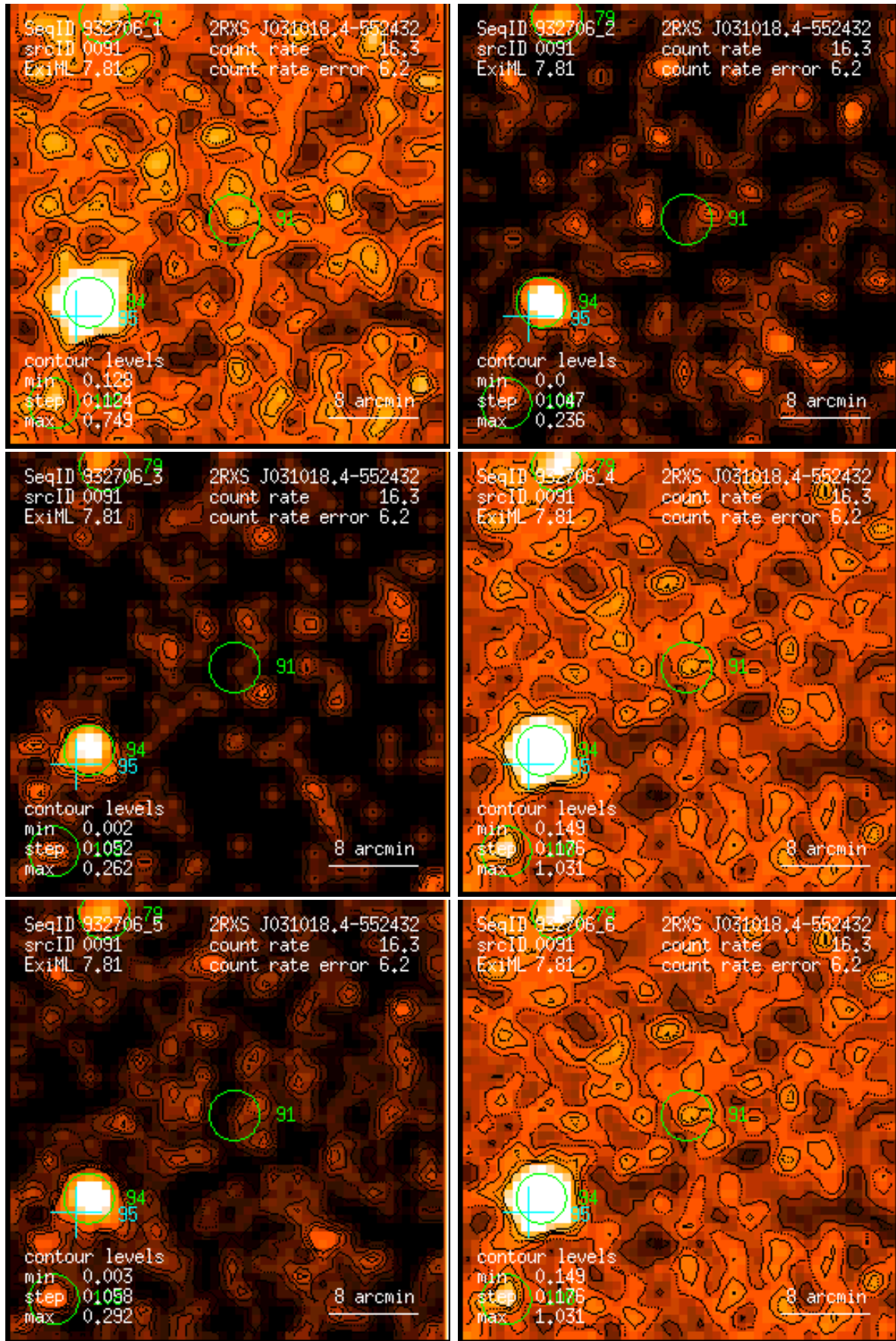
Figure 91: RASS 932706: detection 0091: band rate images, Gaussian filter: (1) PSPC channels 11 – 41, (2) 52 – 90, (3) 91 – 201, (4) 11 – 235, (5) 52 – 201, (6) 11 – 201. Broad band rates in counts/ks. Band rate contour levels in counts/ks/arcmin 2 .
