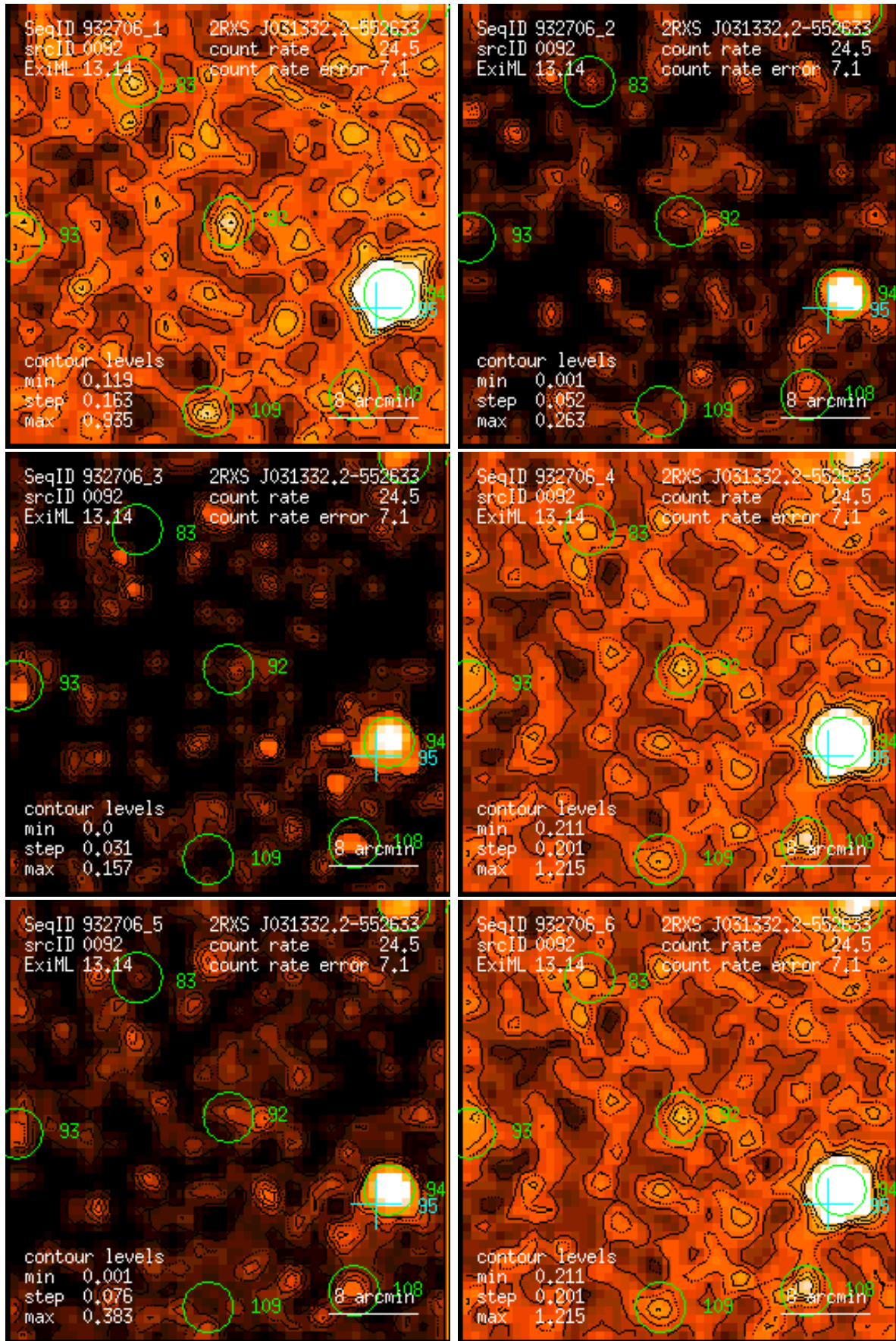
Figure 92: RASS 932706: detection 0092: band rate images, Gaussian filter: (1) PSPC channels 11 – 41, (2) 52 – 90, (3) 91 – 201, (4) 11 – 235, (5) 52 – 201, (6) 11 – 201. Broad band rates in counts/ks. Band rate contour levels in counts/ks/arcmin 2 .
