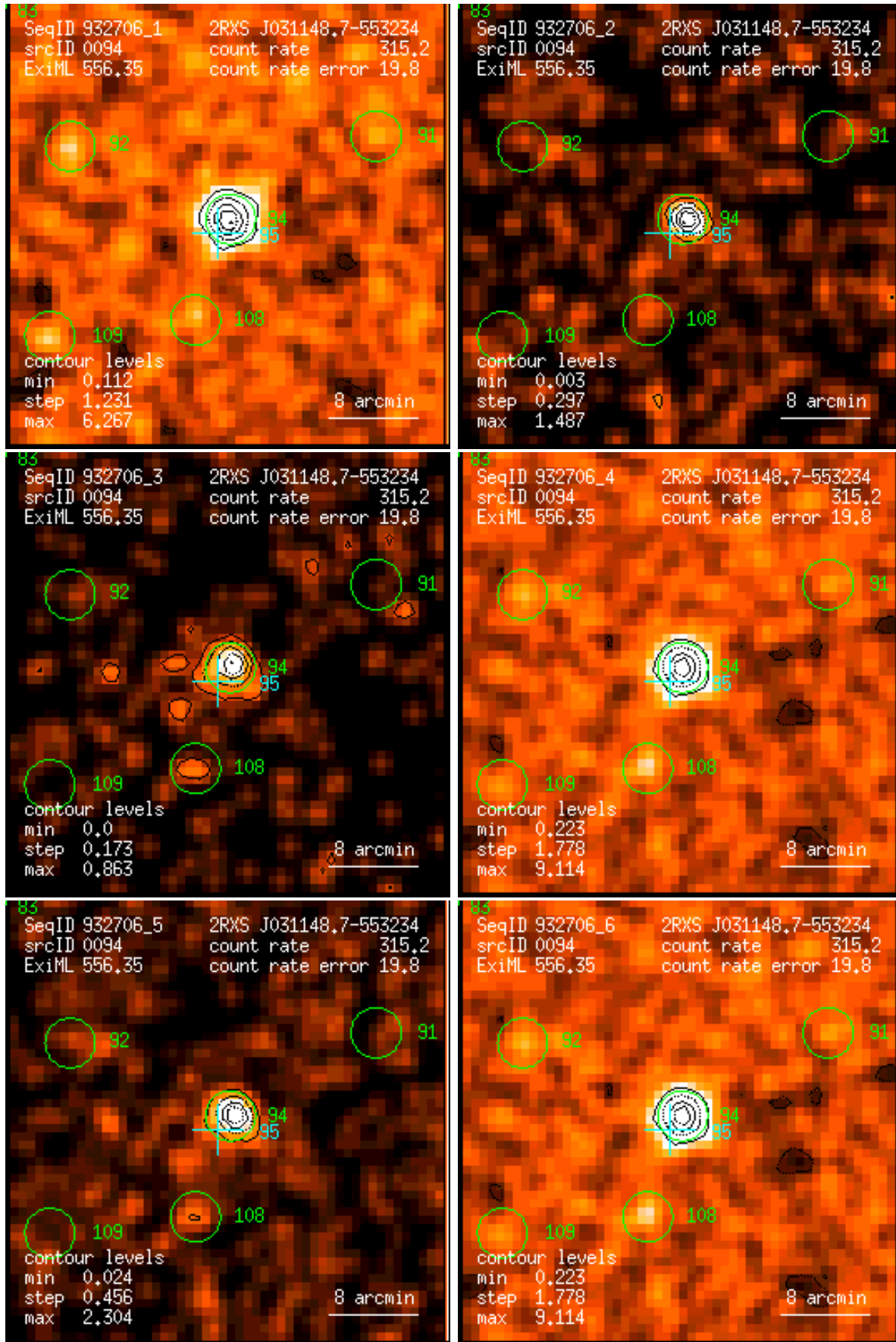
Figure 94: RASS 932706: detection 0094: band rate images, Gaussian filter: (1) PSPC channels 11 – 41, (2) 52 – 90, (3) 91 – 201, (4) 11 – 235, (5) 52 – 201, (6) 11 – 201. Broad band rates in counts/ks. Band rate contour levels in counts/ks/arcmin 2 .
