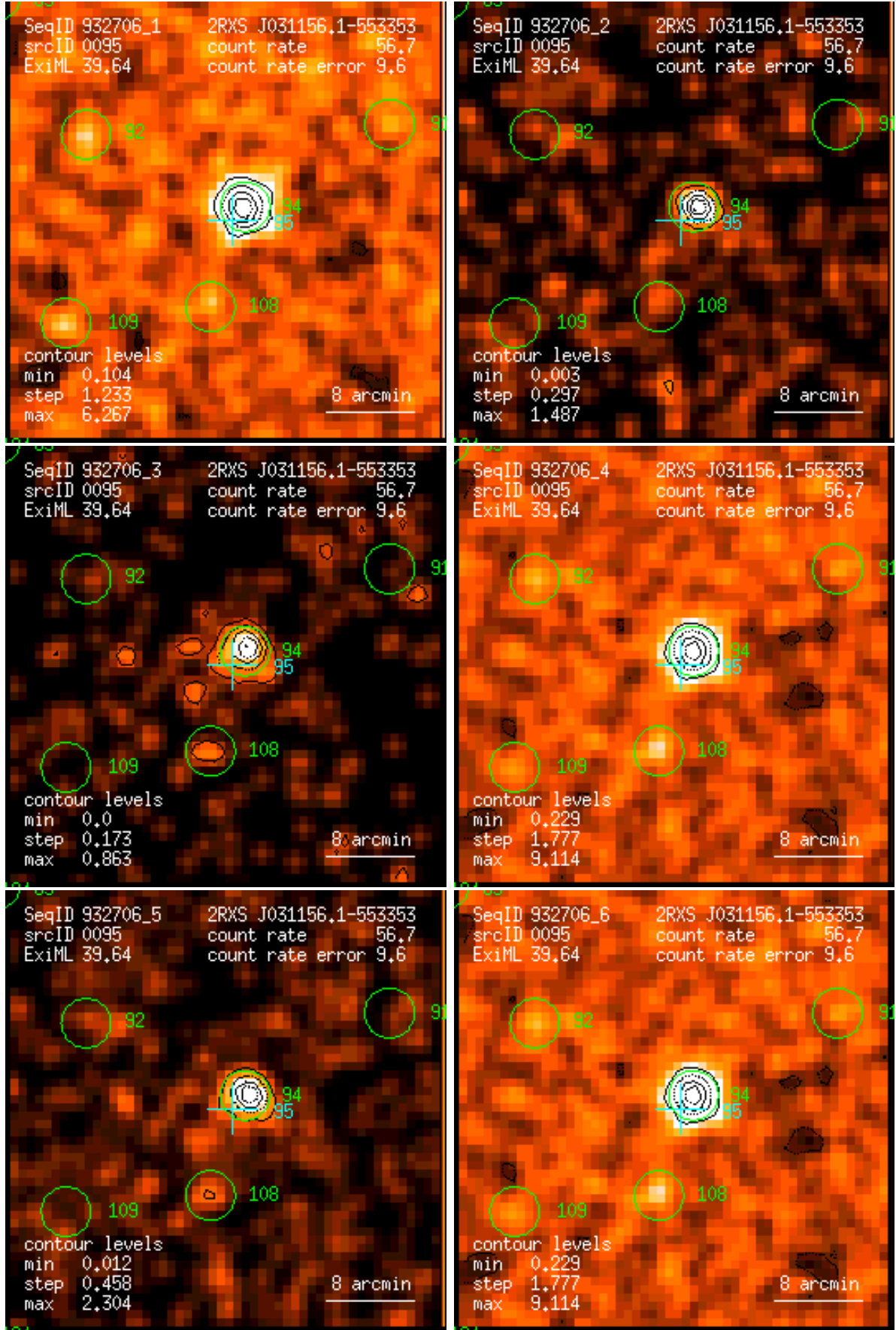
Figure 95: RASS 932706: detection 0095: band rate images, Gaussian filter: (1) PSPC channels 11 – 41, (2) 52 – 90, (3) 91 – 201, (4) 11 – 235, (5) 52 – 201, (6) 11 – 201. Broad band rates in counts/ks. Band rate contour levels in counts/ks/arcmin 2 .
