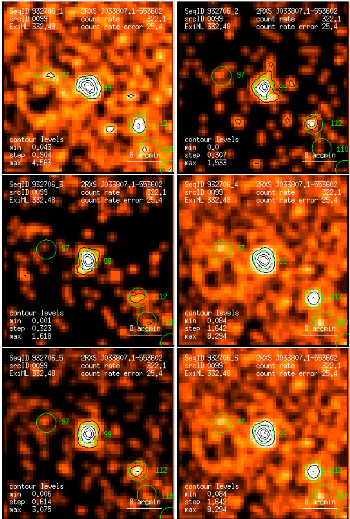
Figure 99: RASS 932706: detection 0099: band rate images, Gaussian filter: (1) PSPC channels 11 – 41, (2) 52 – 90, (3) 91 – 201, (4) 11 – 235, (5) 52 – 201, (6) 11 – 201. Broad band rates in counts/ks. Band rate contour levels in counts/ks/arcmin 2 .
