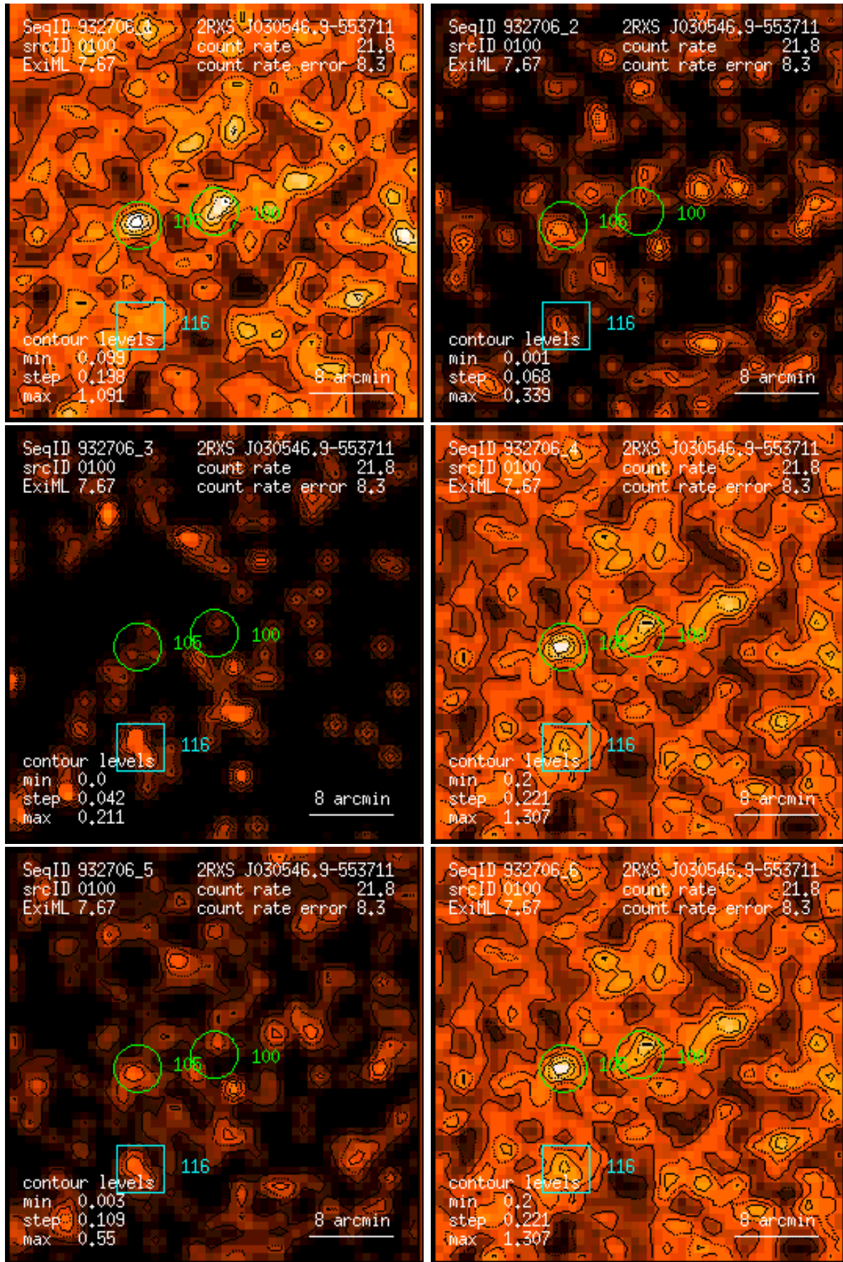
Figure 100: RASS 932706: detection 0100: band rate images, Gaussian filter: (1) PSPC channels 11 – 41, (2) 52 – 90, (3) 91 – 201, (4) 11 – 235, (5) 52 – 201, (6) 11 – 201. Broad band rates in counts/ks. Band rate contour levels in counts/ks/arcmin 2 .
