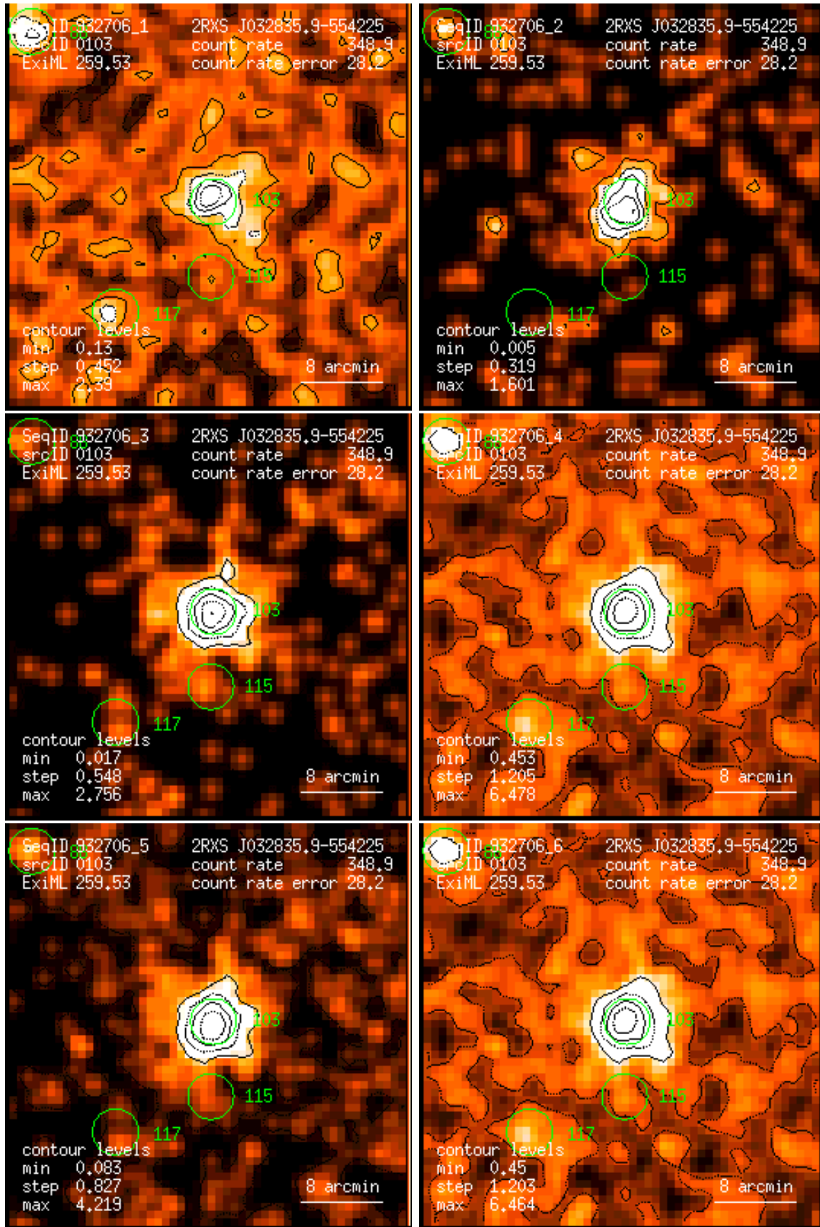
Figure 103: RASS 932706: detection 0103: band rate images, Gaussian filter: (1) PSPC channels 11 – 41, (2) 52 – 90, (3) 91 – 201, (4) 11 – 235, (5) 52 – 201, (6) 11 – 201. Broad band rates in counts/ks. Band rate contour levels in counts/ks/arcmin 2 .
