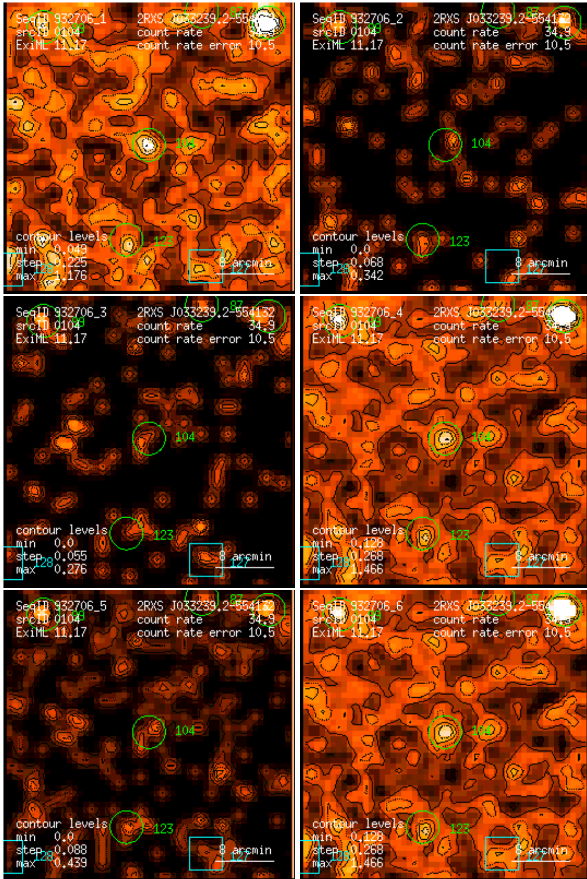
Figure 104: RASS 932706: detection 0104: band rate images, Gaussian filter: (1) PSPC channels 11 – 41, (2) 52 – 90, (3) 91 – 201, (4) 11 – 235, (5) 52 – 201, (6) 11 – 201. Broad band rates in counts/ks. Band rate contour levels in counts/ks/arcmin 2 .
