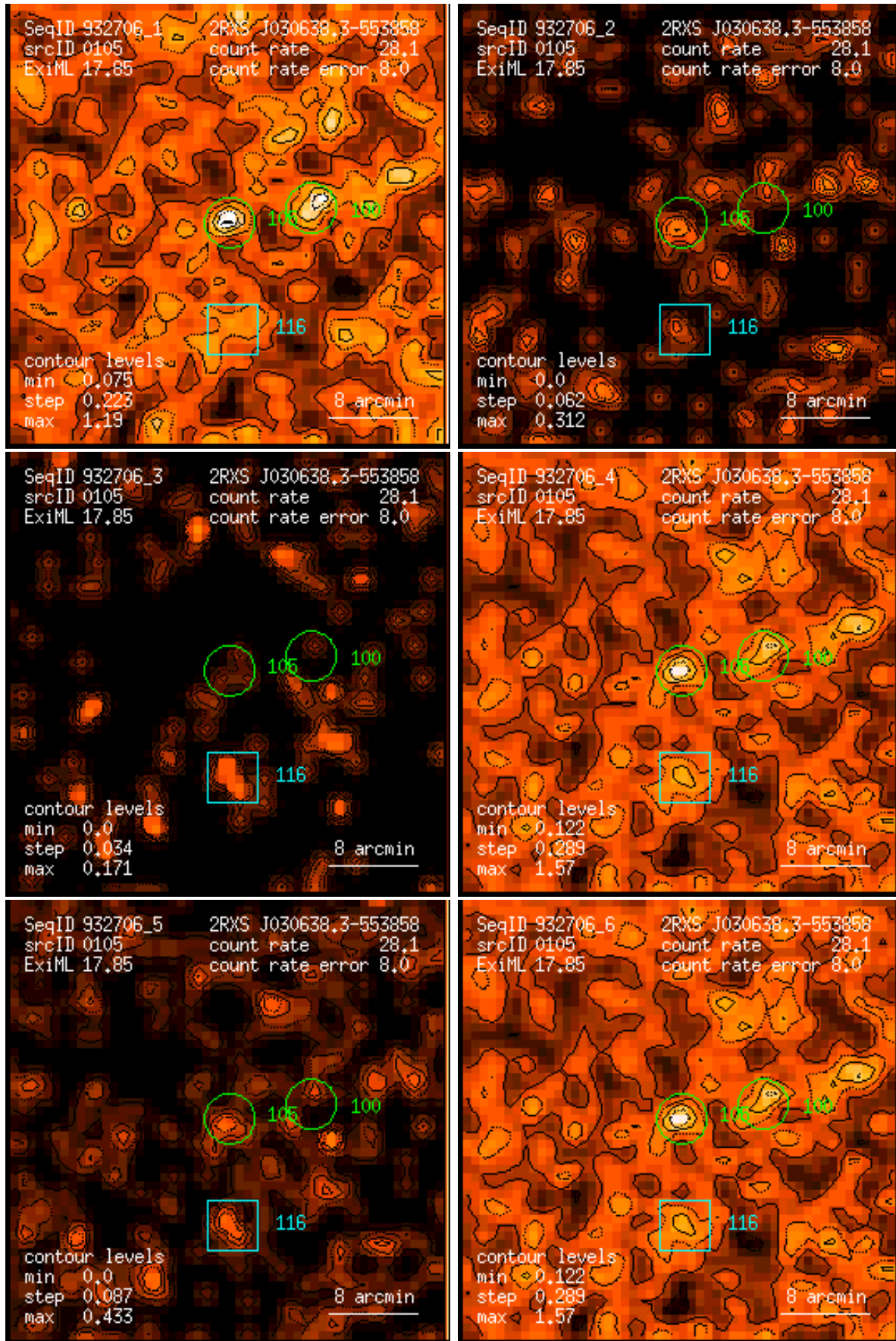
Figure 105: RASS 932706: detection 0105: band rate images, Gaussian filter: (1) PSPC channels 11 – 41, (2) 52 – 90, (3) 91 – 201, (4) 11 – 235, (5) 52 – 201, (6) 11 – 201. Broad band rates in counts/ks. Band rate contour levels in counts/ks/arcmin 2 .
