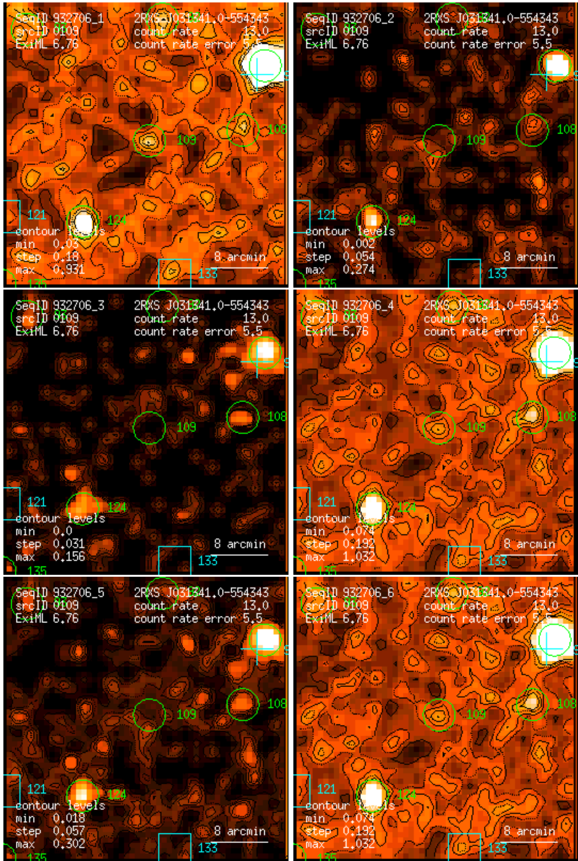
Figure 109: RASS 932706: detection 0109: band rate images, Gaussian filter: (1) PSPC channels 11 – 41, (2) 52 – 90, (3) 91 – 201, (4) 11 – 235, (5) 52 – 201, (6) 11 – 201. Broad band rates in counts/ks. Band rate contour levels in counts/ks/arcmin 2 .
