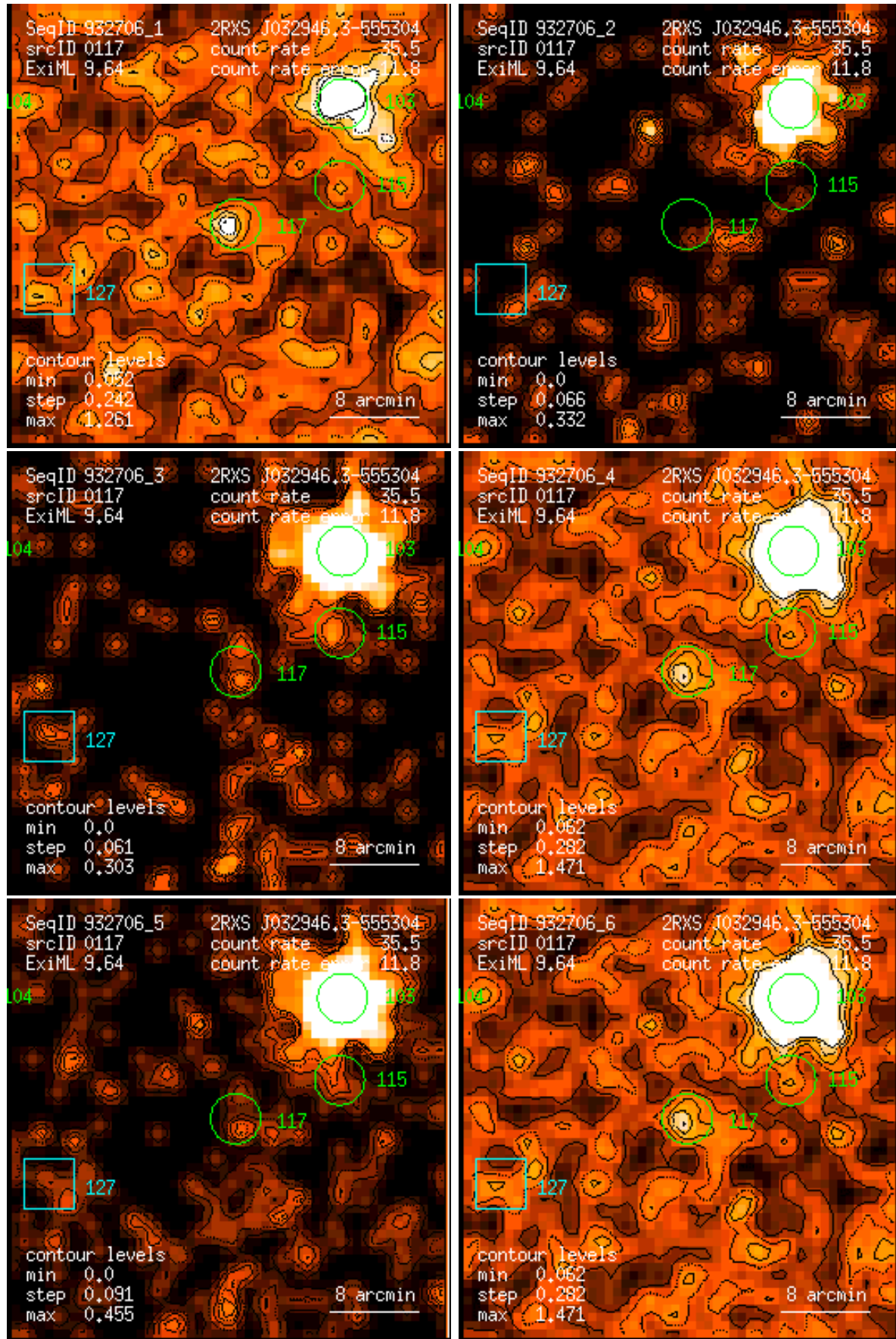
Figure 117: RASS 932706: detection 0117: band rate images, Gaussian filter: (1) PSPC channels 11 – 41, (2) 52 – 90, (3) 91 – 201, (4) 11 – 235, (5) 52 – 201, (6) 11 – 201. Broad band rates in counts/ks. Band rate contour levels in counts/ks/arcmin 2 .
