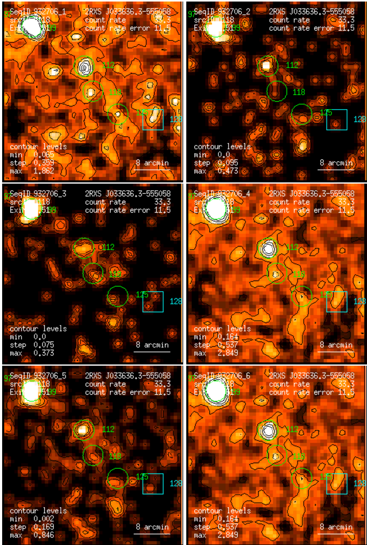
Figure 118: RASS 932706: detection 0118: band rate images, Gaussian filter: (1) PSPC channels 11 – 41, (2) 52 – 90, (3) 91 – 201, (4) 11 – 235, (5) 52 – 201, (6) 11 – 201. Broad band rates in counts/ks. Band rate contour levels in counts/ks/arcmin 2 .
