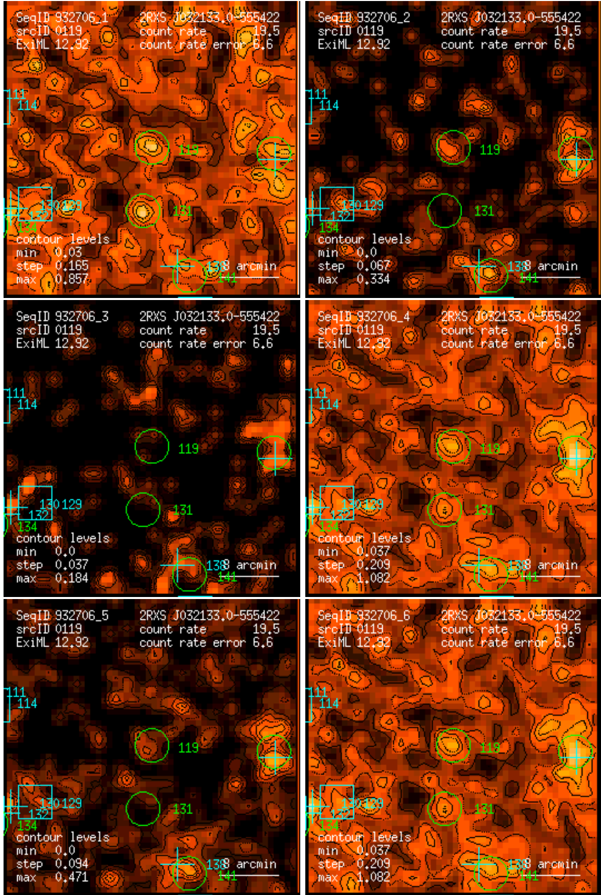
Figure 119: RASS 932706: detection 0119: band rate images, Gaussian filter: (1) PSPC channels 11 – 41, (2) 52 – 90, (3) 91 – 201, (4) 11 – 235, (5) 52 – 201, (6) 11 – 201. Broad band rates in counts/ks. Band rate contour levels in counts/ks/arcmin 2 .
