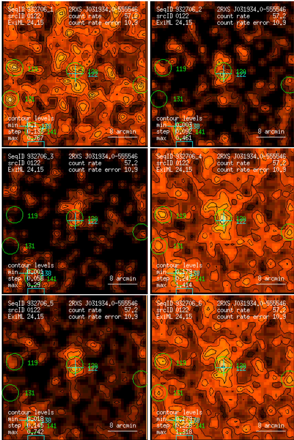
Figure 122: RASS 932706: detection 0122: band rate images, Gaussian filter: (1) PSPC channels 11 – 41, (2) 52 – 90, (3) 91 – 201, (4) 11 – 235, (5) 52 – 201, (6) 11 – 201. Broad band rates in counts/ks. Band rate contour levels in counts/ks/arcmin 2 .
