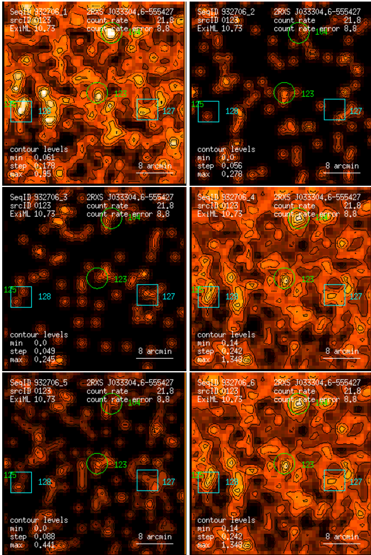
Figure 123: RASS 932706: detection 0123: band rate images, Gaussian filter: (1) PSPC channels 11 – 41, (2) 52 – 90, (3) 91 – 201, (4) 11 – 235, (5) 52 – 201, (6) 11 – 201. Broad band rates in counts/ks. Band rate contour levels in counts/ks/arcmin 2 .
