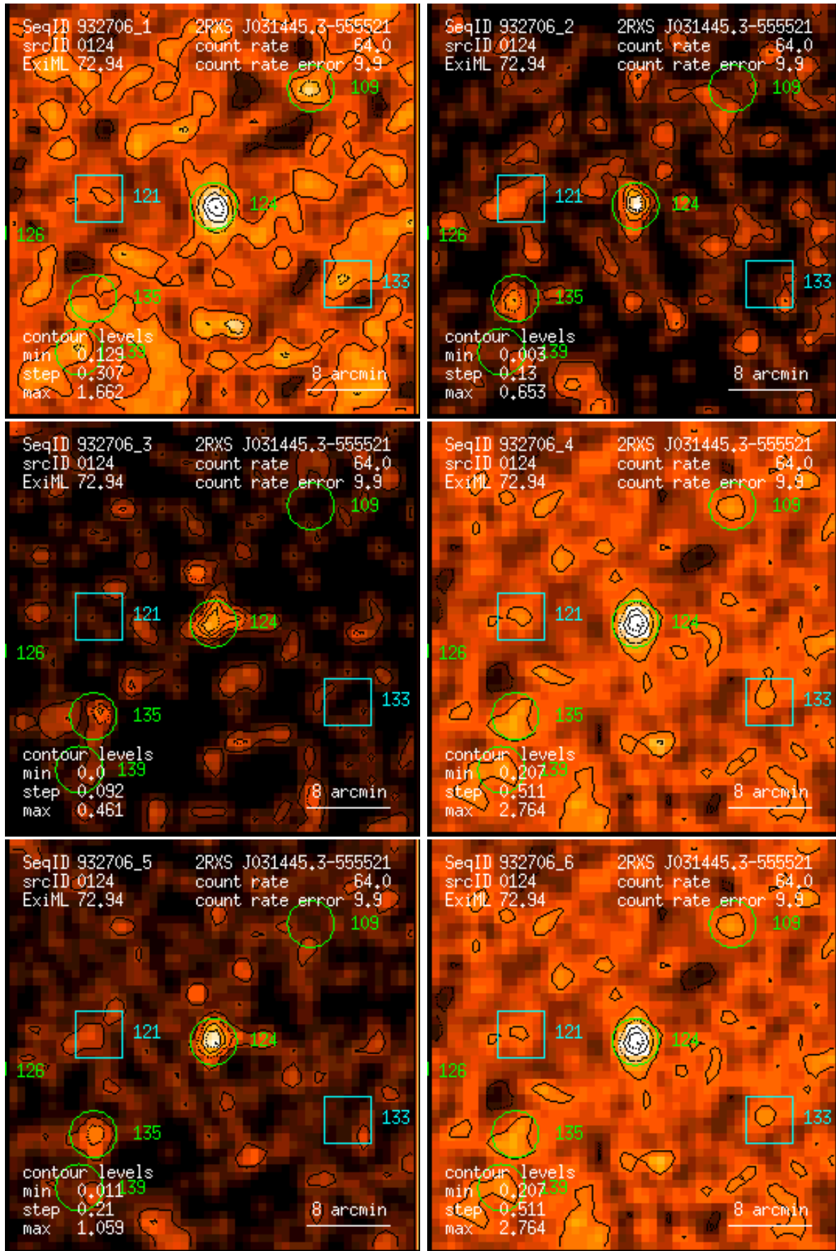
Figure 124: RASS 932706: detection 0124: band rate images, Gaussian filter: (1) PSPC channels 11 – 41, (2) 52 – 90, (3) 91 – 201, (4) 11 – 235, (5) 52 – 201, (6) 11 – 201. Broad band rates in counts/ks. Band rate contour levels in counts/ks/arcmin 2 .
