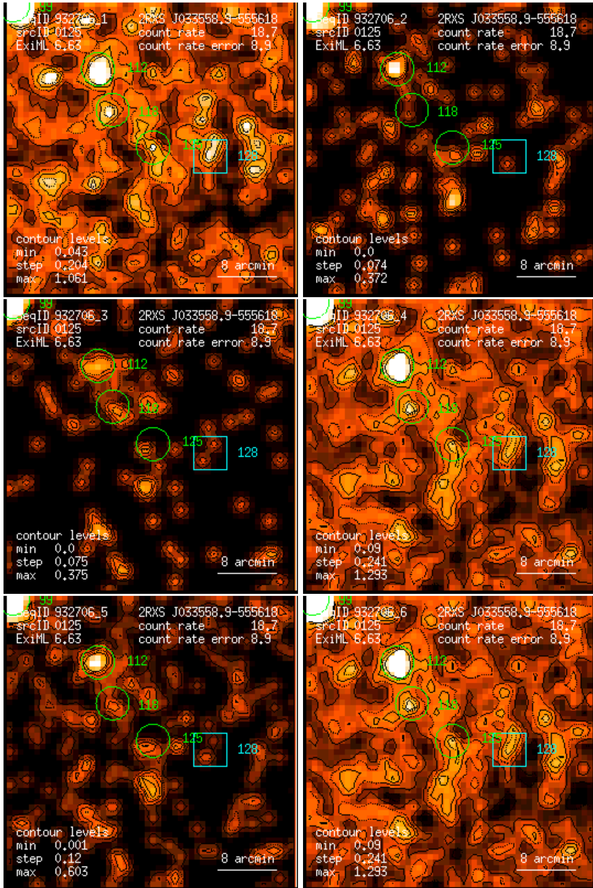
Figure 125: RASS 932706: detection 0125: band rate images, Gaussian filter: (1) PSPC channels 11 – 41, (2) 52 – 90, (3) 91 – 201, (4) 11 – 235, (5) 52 – 201, (6) 11 – 201. Broad band rates in counts/ks. Band rate contour levels in counts/ks/arcmin 2 .
