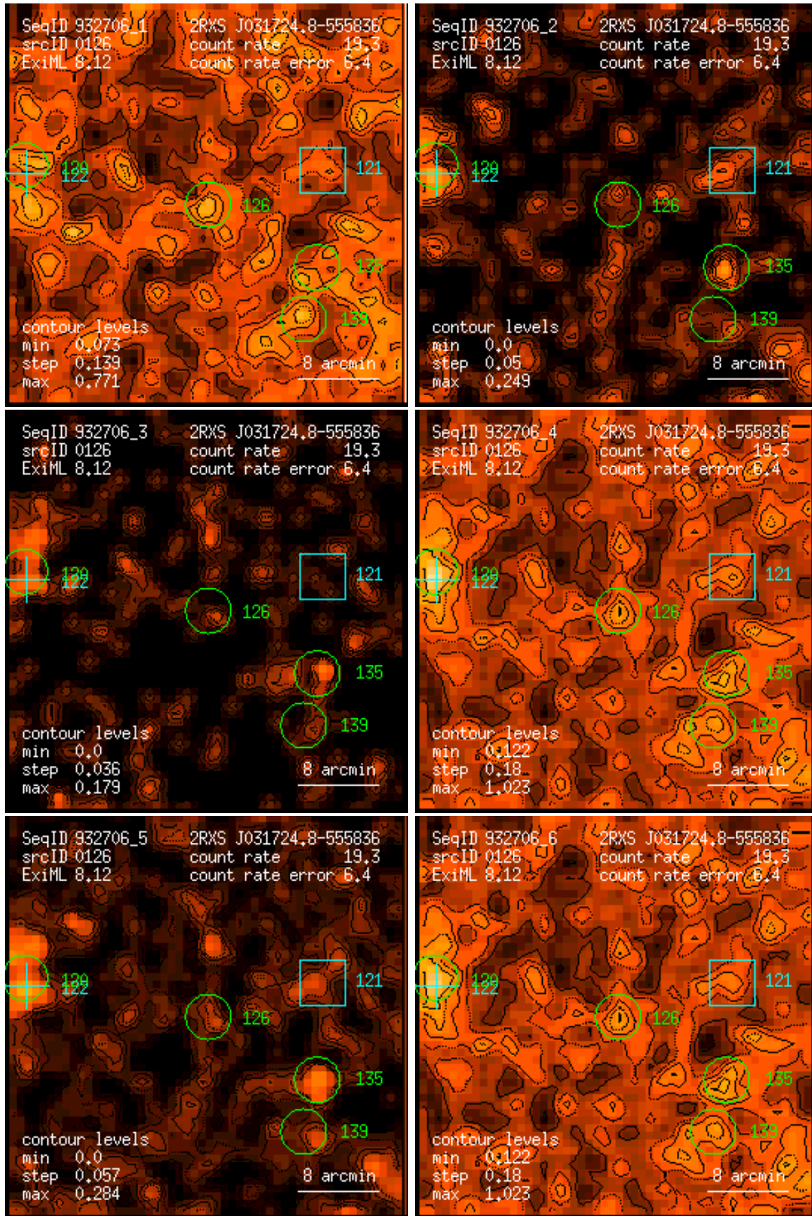
Figure 126: RASS 932706: detection 0126: band rate images, Gaussian filter: (1) PSPC channels 11 – 41, (2) 52 – 90, (3) 91 – 201, (4) 11 – 235, (5) 52 – 201, (6) 11 – 201. Broad band rates in counts/ks. Band rate contour levels in counts/ks/arcmin 2 .
